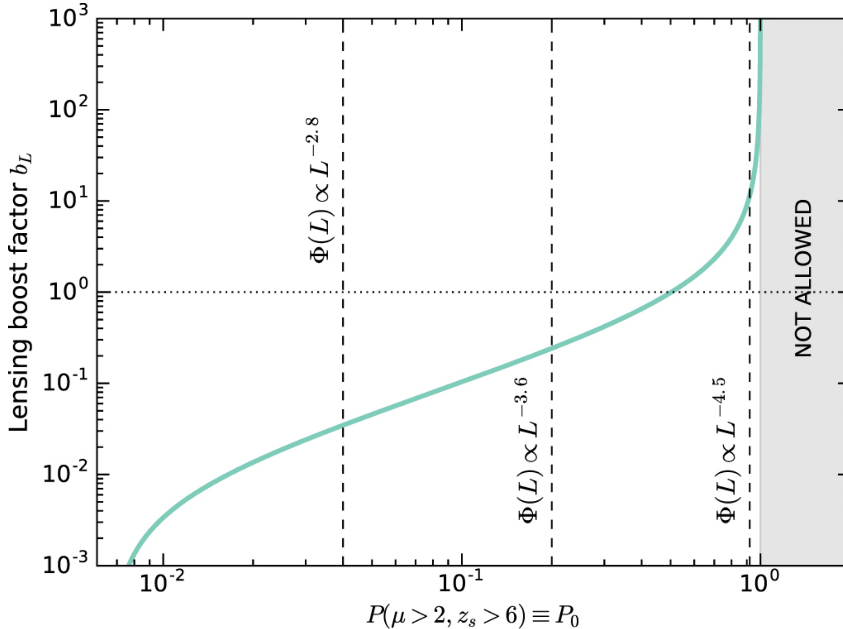
Figure 3. from Most Lensed Quasars at z > 6 are Missed by Current Surveys null 2019 APJL 870 L12 doi:10.3847/2041-8213/aaf86a http://dx.doi.org/10.3847/2041-8213/aaf86a © 2019. The American Astronomical Society. All rights reserved.
