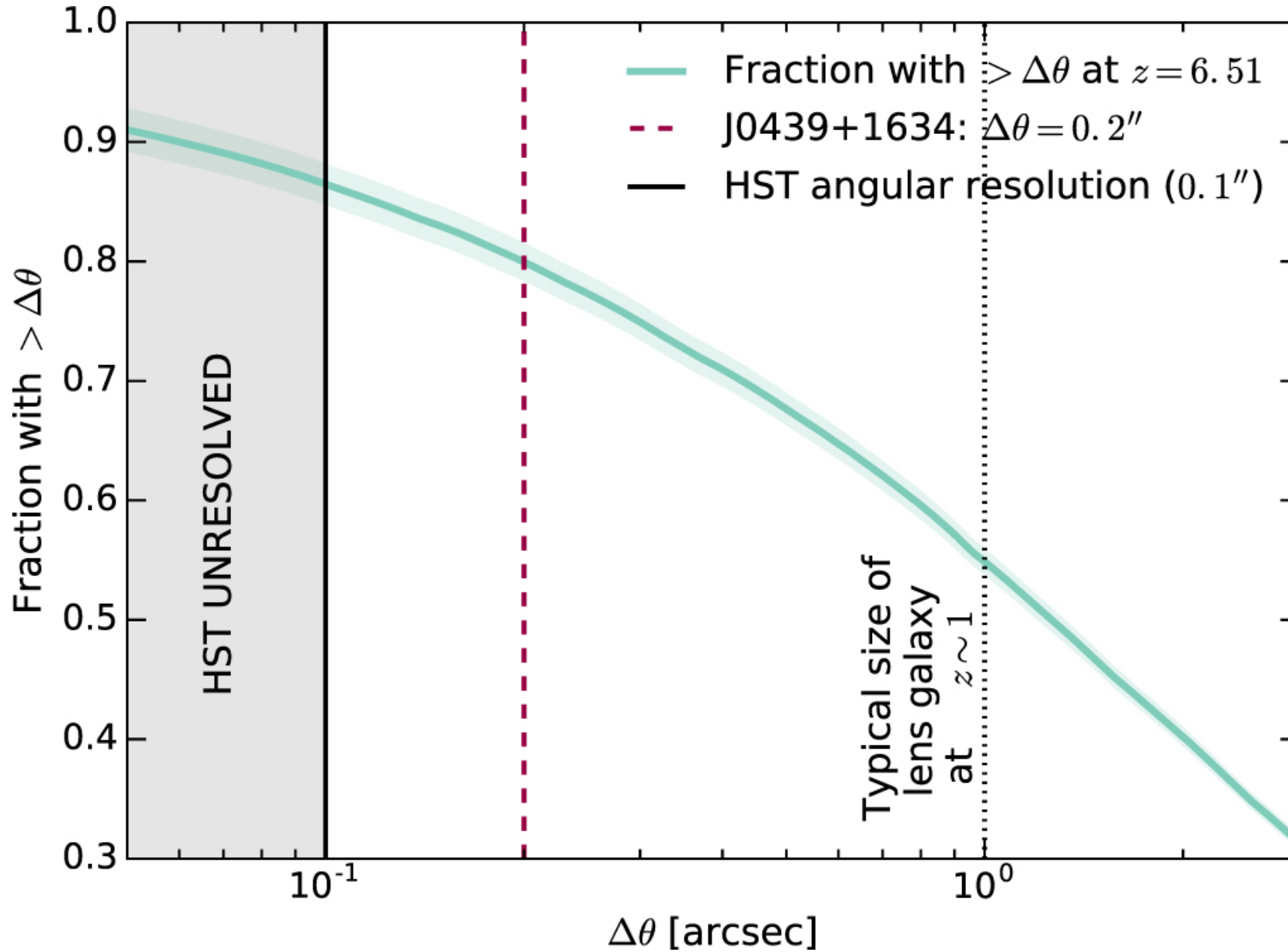
Figure 2. from Most Lensed Quasars at z > 6 are Missed by Current Surveys null 2019 APJL 870 L12 doi:10.3847/2041-8213/aaf86a http://dx.doi.org/10.3847/2041-8213/aaf86a © 2019. The American Astronomical Society. All rights reserved.
