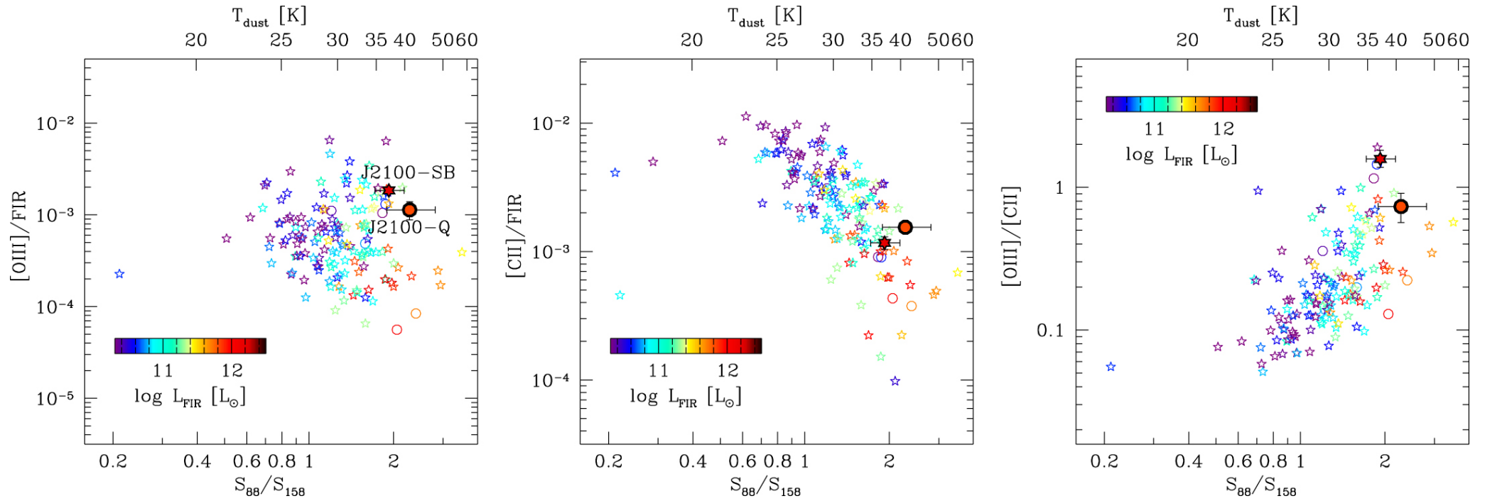
Figure 4. from No Evidence for Enhanced [O III] 88 m Emission in a z \sim 6 Quasar Compared to Its Companion Starbursting Galaxy null 2018 APJL 869 L22 doi:10.3847/2041-8213/aaf4fa https://dx.doi.org/10.3847/2041-8213/aaf4fa © 2018. The American Astronomical Society. All rights reserved.
