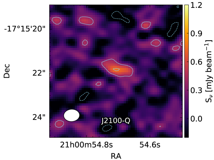
Figure 3. from No Evidence for Enhanced [O III] 88 m Emission in a z \sim 6 Quasar Compared to Its Companion Starbursting Galaxy null 2018 APJL 869 L22 doi:10.3847/2041-8213/aaf4fa https://dx.doi.org/10.3847/2041-8213/aaf4fa © 2018. The American Astronomical Society. All rights reserved.
