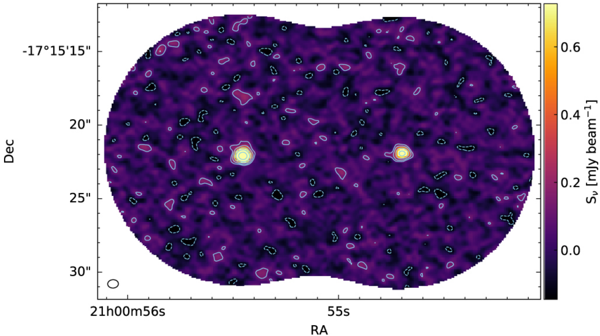
Figure 1. from No Evidence for Enhanced [O III] 88 m Emission in a z \sim 6 Quasar Compared to Its Companion Starbursting Galaxy null 2018 APJL 869 L22 doi:10.3847/2041-8213/aaf4fa https://dx.doi.org/10.3847/2041-8213/aaf4fa © 2018. The American Astronomical Society. All rights reserved.
