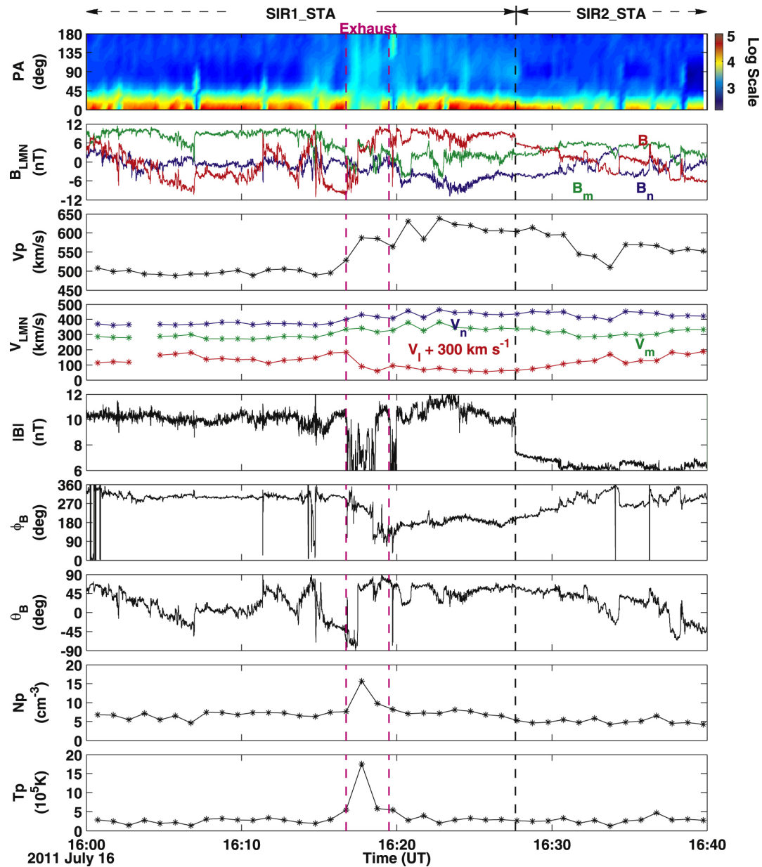
Figure 5. from The Merging of Two Stream Interaction Regions within 1 au: The Possible Role of Magnetic Reconnection null 2018 APJL 869 L6 doi:10.3847/2041-8213/aaf398 https://dx.doi.org/10.3847/2041-8213/aaf398 © 2018. The American Astronomical Society. All rights reserved.
