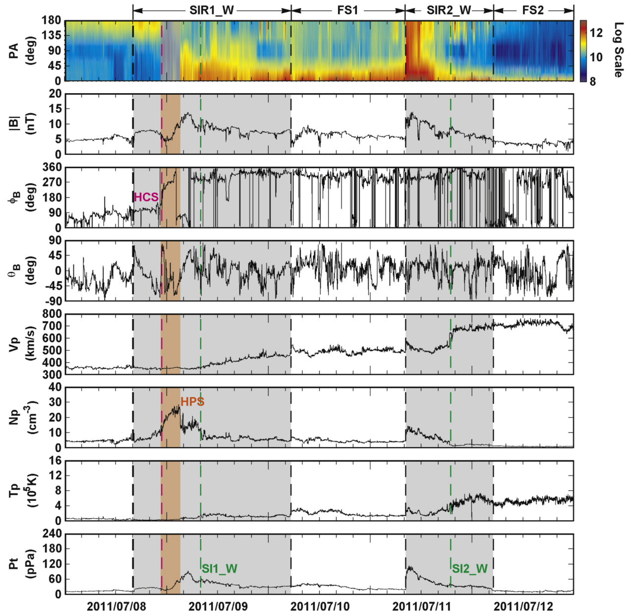
Figure 2. from The Merging of Two Stream Interaction Regions within 1 au: The Possible Role of Magnetic Reconnection null 2018 APJL 869 L6 doi:10.3847/2041-8213/aaf398 https://dx.doi.org/10.3847/2041-8213/aaf398 © 2018. The American Astronomical Society. All rights reserved.
