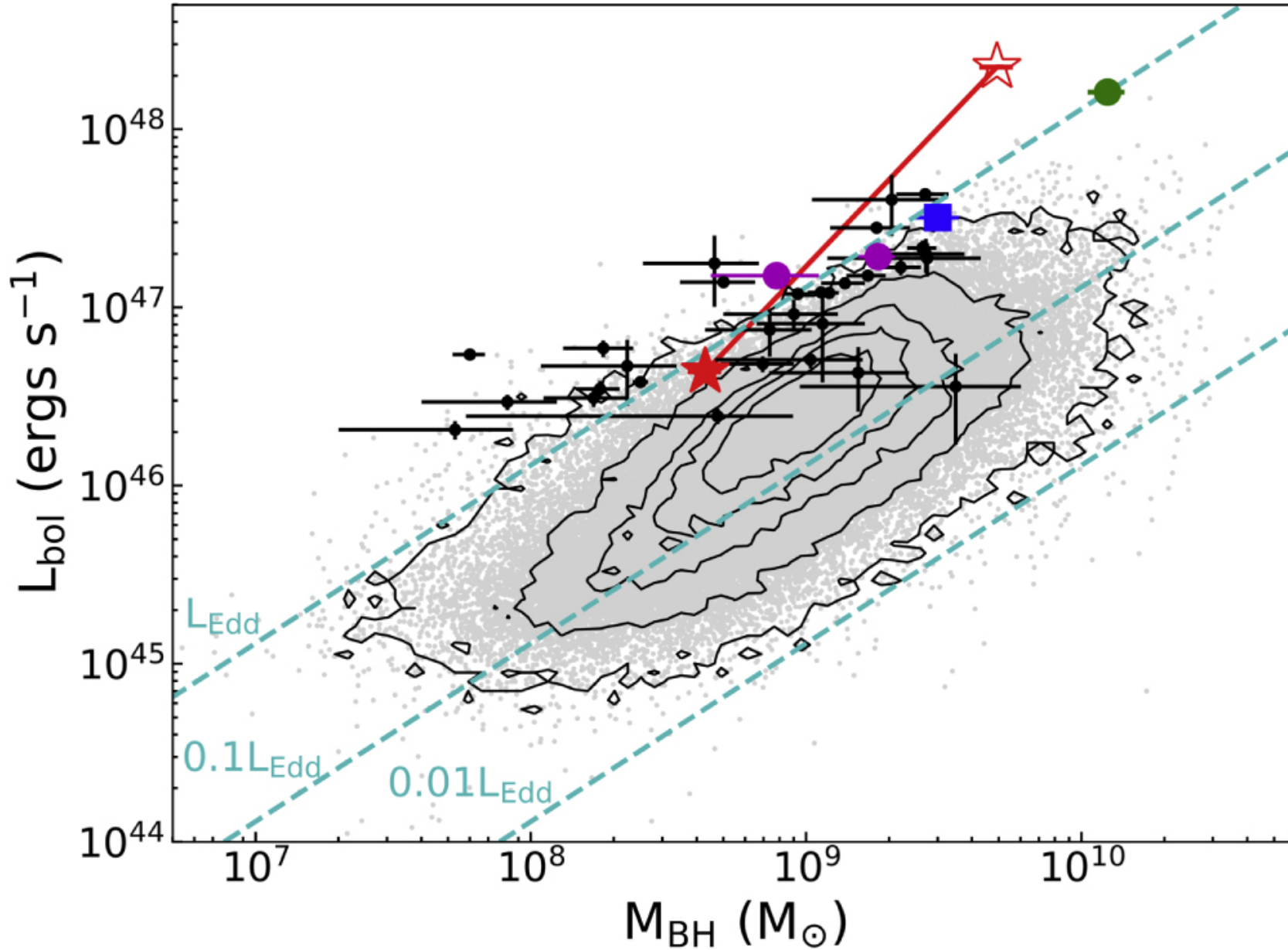
Figure 2. from The Discovery of a Gravitationally Lensed Quasar at z = 6.51 null 2019 APJL 870 L11 doi:10.3847/2041-8213/aaeffe http://dx.doi.org/10.3847/2041-8213/aaeffe © 2019. The American Astronomical Society. All rights reserved.
