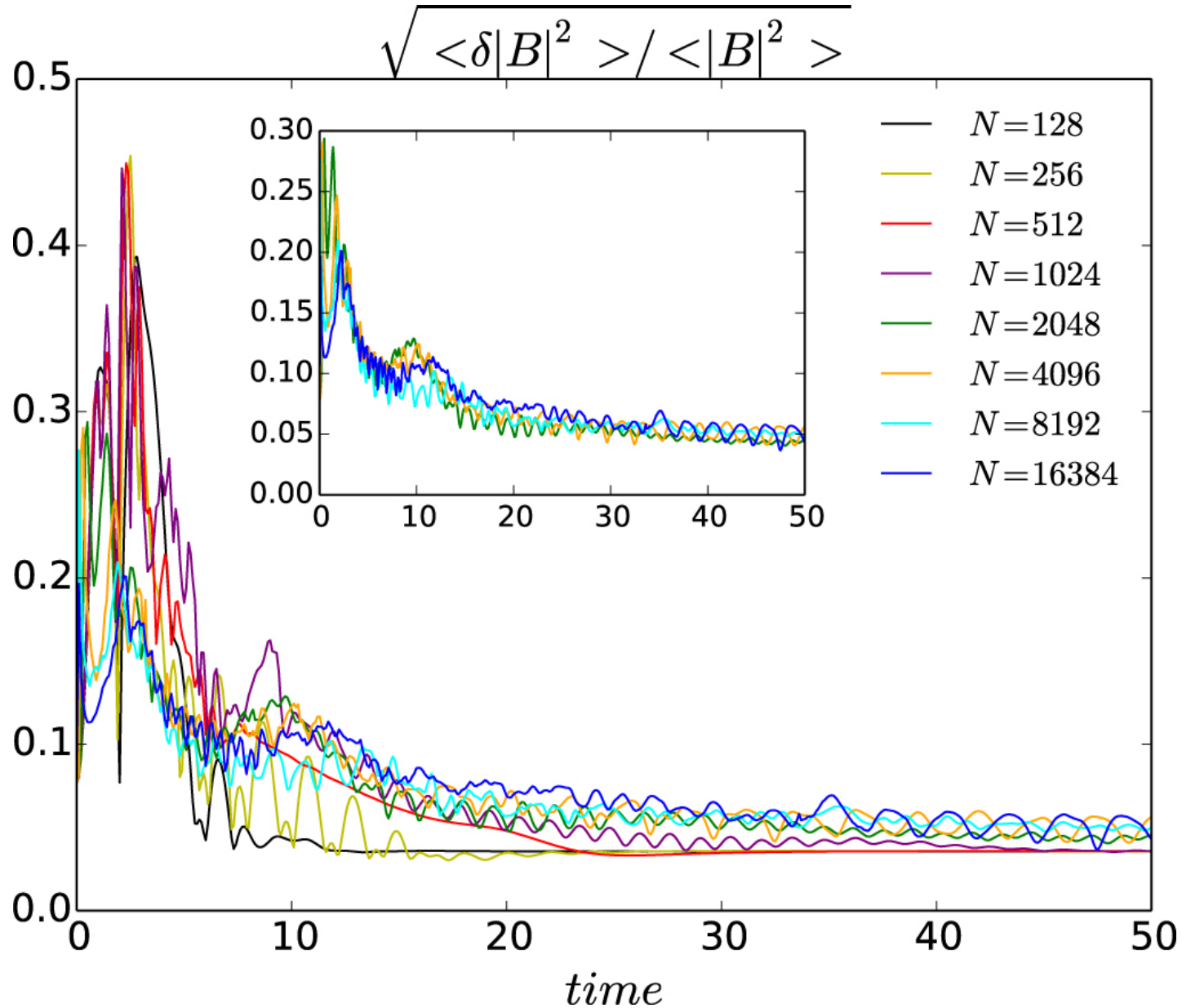
Figure 1. from Nonlinear Firehose Relaxation and Constant-B Field Fluctuations null 2018 APJL 867 L26 doi:10.3847/2041-8213/aaec01 http://dx.doi.org/10.3847/2041-8213/aaec01 © 2018. The American Astronomical Society. All rights reserved.
