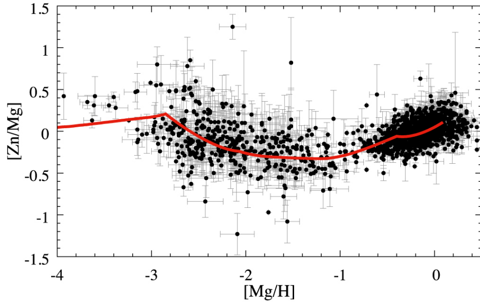
Figure 4. from Early Chemical Evolution of Zn Driven by Magnetorotational Supernovae and the Pathway to the Solar Zn Composition null 2018 APJL 863 L27 doi:10.3847/2041-8213/aad86b https://dx.doi.org/10.3847/2041-8213/aad86b © 2018. The American Astronomical Society. All rights reserved.
