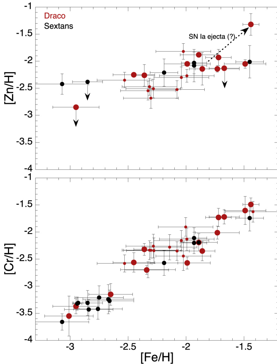
Figure 2. from Early Chemical Evolution of Zn Driven by Magnetorotational Supernovae and the Pathway to the Solar Zn Composition null 2018 APJL 863 L27 doi:10.3847/2041-8213/aad86b https://dx.doi.org/10.3847/2041-8213/aad86b © 2018. The American Astronomical Society. All rights reserved.
