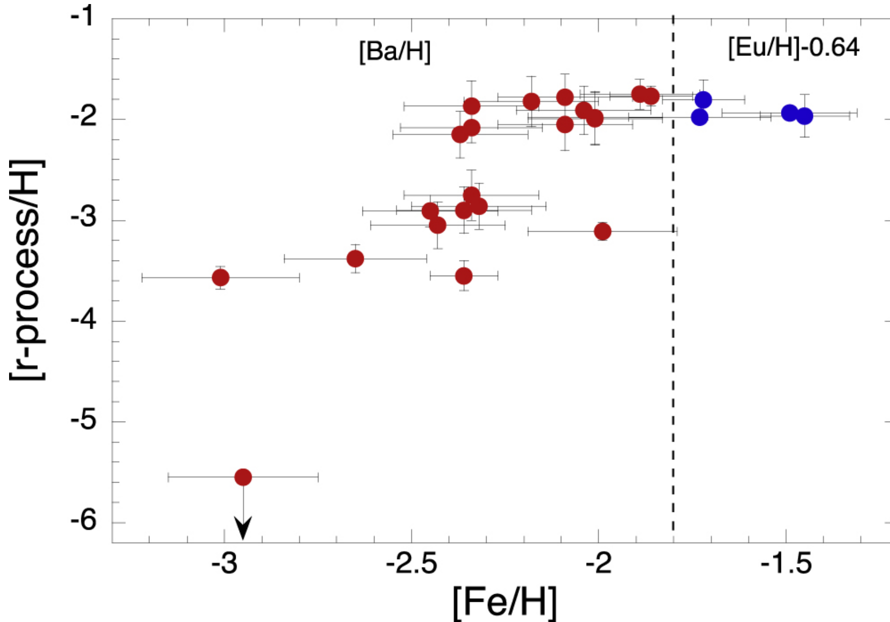
Figure 1. from Early Chemical Evolution of Zn Driven by Magnetorotational Supernovae and the Pathway to the Solar Zn Composition null 2018 APJL 863 L27 doi:10.3847/2041-8213/aad86b https://dx.doi.org/10.3847/2041-8213/aad86b © 2018. The American Astronomical Society. All rights reserved.
