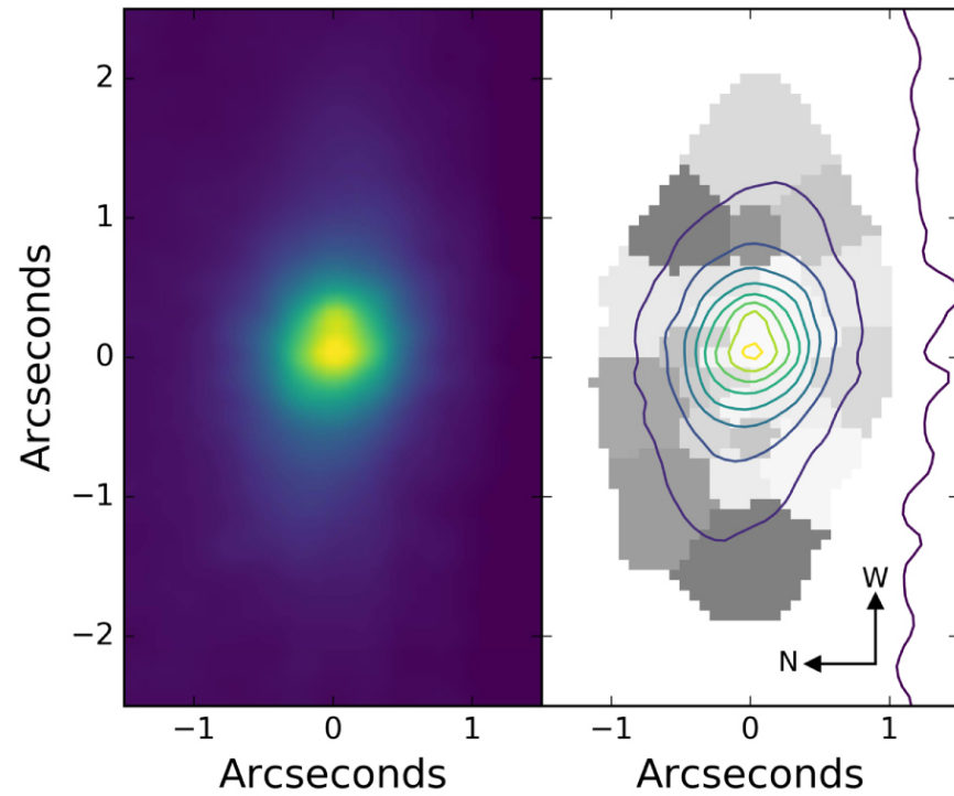
(a) Flux density of SDSS J0912+1523
