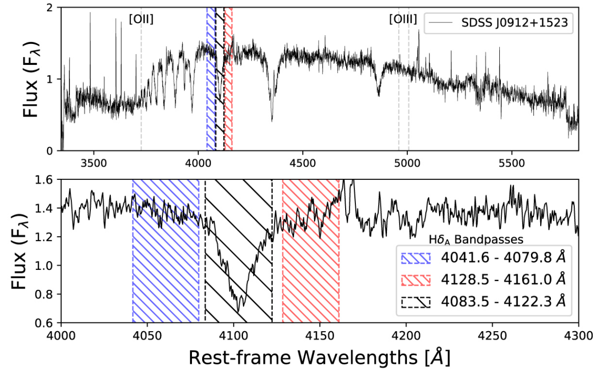
(b) Central spectrum and H\delta_A bandpasses
