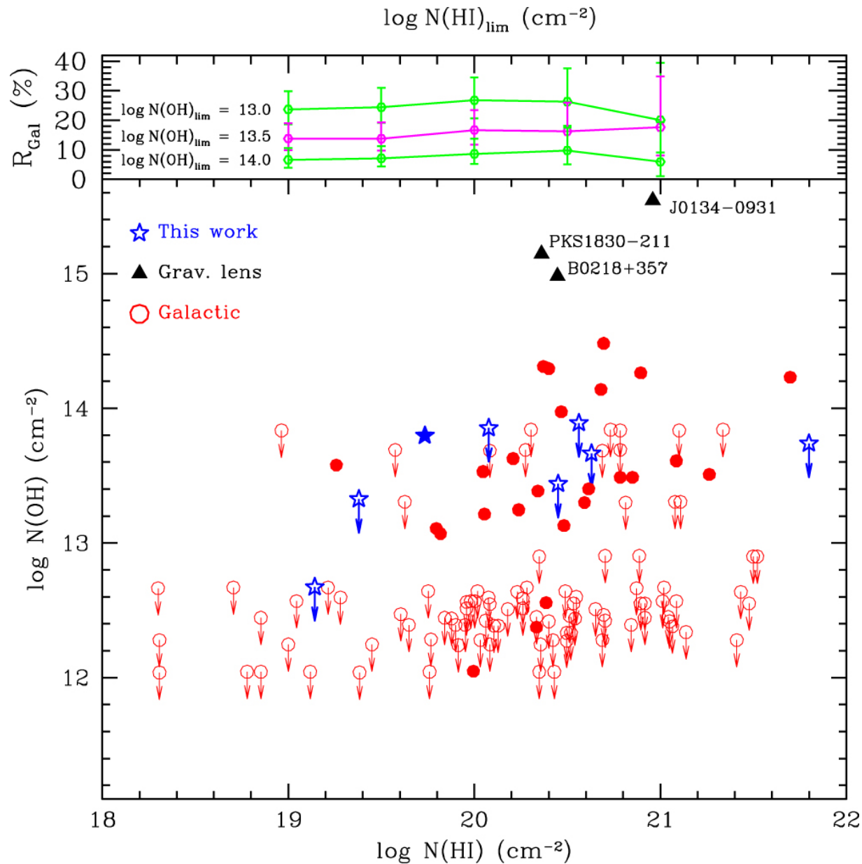
Figure 3. from Discovery of OH Absorption from a Galaxy at z = 0.05 : Implications for Large Surveys with SKA Pathfinders null 2018 APJL 860 L22 doi:10.3847/2041-8213/aac9cd https://dx.doi.org/10.3847/2041-8213/aac9cd © 2018. The American Astronomical Society. All rights reserved.
