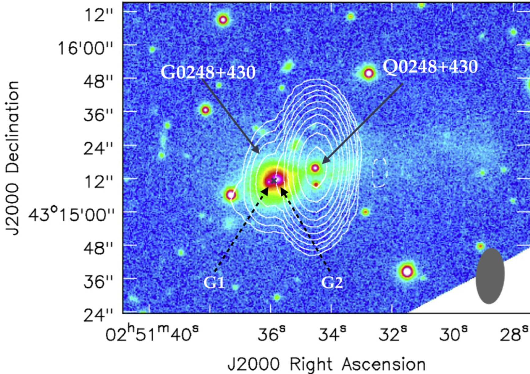
Figure 1. from Discovery of OH Absorption from a Galaxy at z = 0.05 : Implications for Large Surveys with SKA Pathfinders null 2018 APJL 860 L22 doi:10.3847/2041-8213/aac9cd https://dx.doi.org/10.3847/2041-8213/aac9cd © 2018. The American Astronomical Society. All rights reserved.
