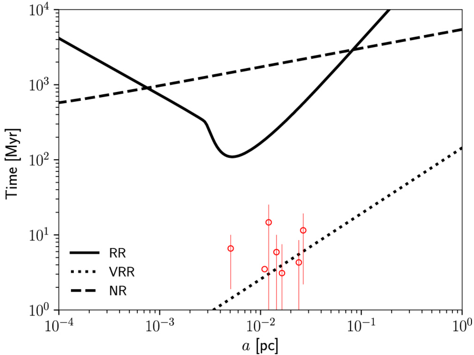
Figure 4. from Scalar Resonant Relaxation of Stars around a Massive Black Hole null 2018 APJL 860 L23 doi:10.3847/2041-8213/aac88e https://dx.doi.org/10.3847/2041-8213/aac88e © 2018. The American Astronomical Society.
