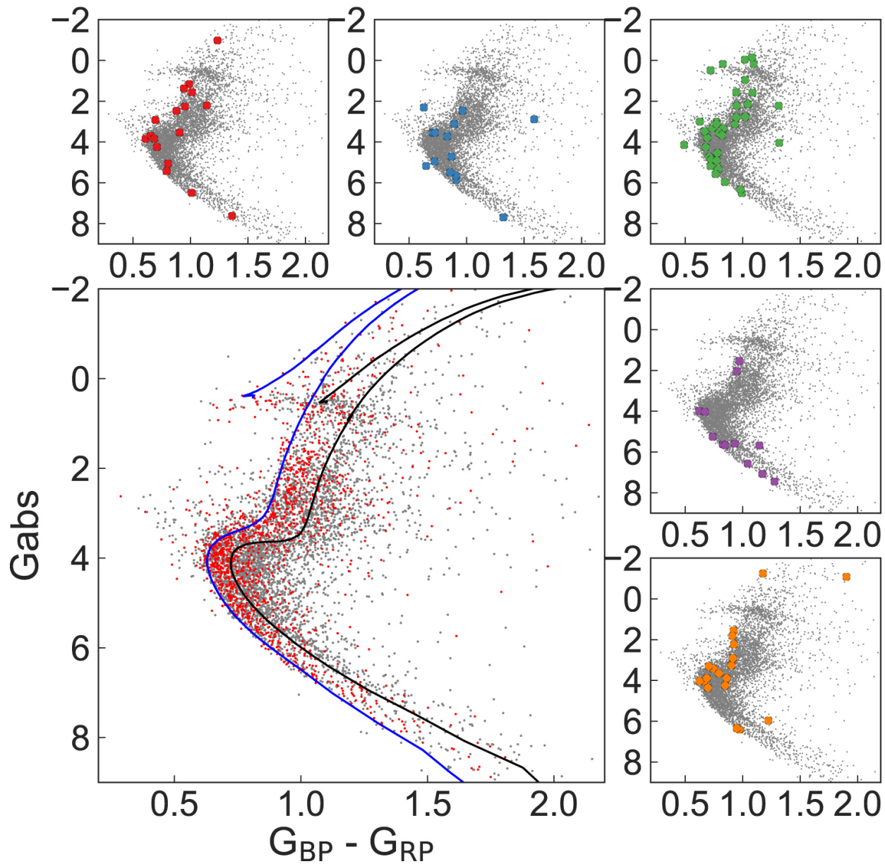
Figure 5. from One Large Blob and Many Streams Frosting the nearby Stellar Halo in Gaia DR2 null 2018 APJL 860 L11 doi:10.3847/2041-8213/aac882 https://dx.doi.org/10.3847/2041-8213/aac882 © 2018. The American Astronomical Society. All rights reserved.
