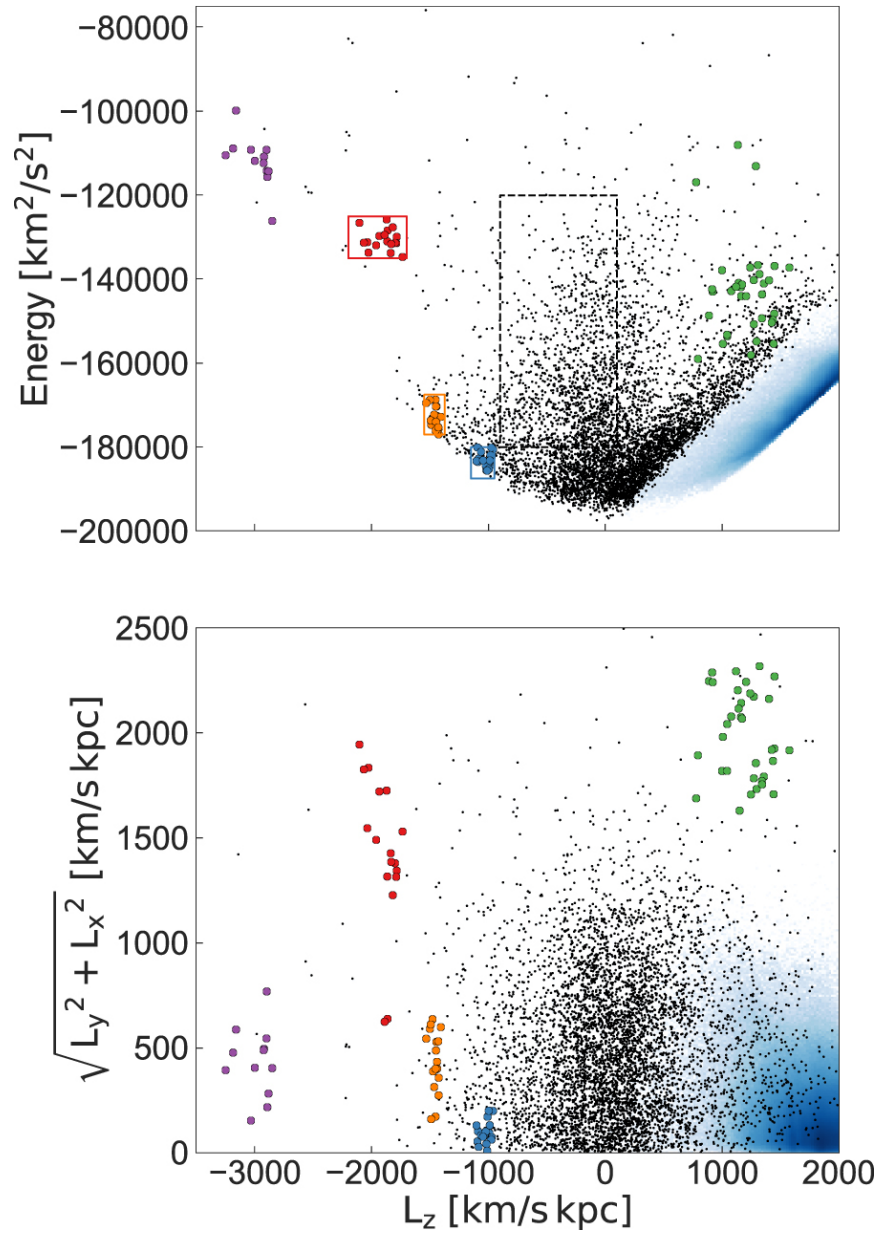
Figure 4. from One Large Blob and Many Streams Frosting the nearby Stellar Halo in Gaia DR2 null 2018 APJL 860 L11 doi:10.3847/2041-8213/aac882 https://dx.doi.org/10.3847/2041-8213/aac882 © 2018. The American Astronomical Society. All rights reserved.
