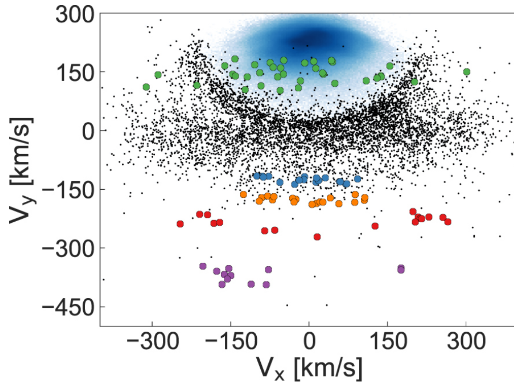
Figure 2. from One Large Blob and Many Streams Frosting the nearby Stellar Halo in Gaia DR2 null 2018 APJL 860 L11 doi:10.3847/2041-8213/aac882 https://dx.doi.org/10.3847/2041-8213/aac882 © 2018. The American Astronomical Society. All rights reserved.
