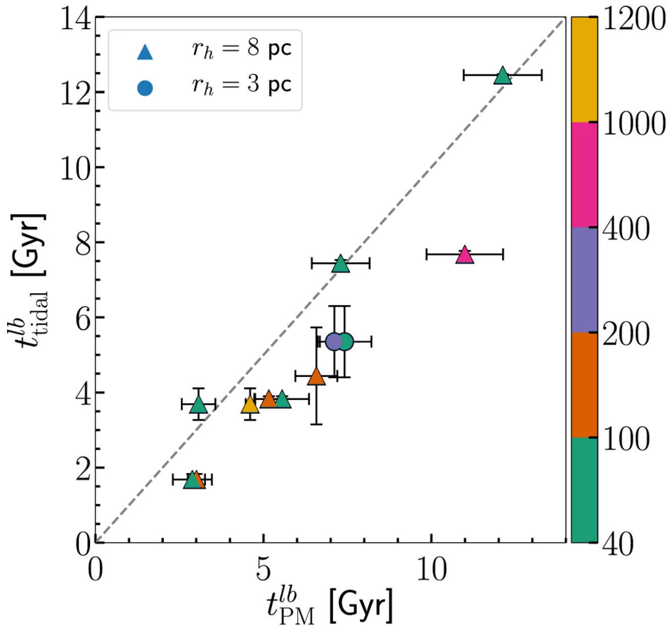
Figure 4. from Dating the Tidal Disruption of Globular Clusters with GAIA Data on Their Stellar Streams null 2018 APJL 859 L13 doi:10.3847/2041-8213/aac48c https://dx.doi.org/10.3847/2041-8213/aac48c © 2018. The American Astronomical Society. All rights reserved.
