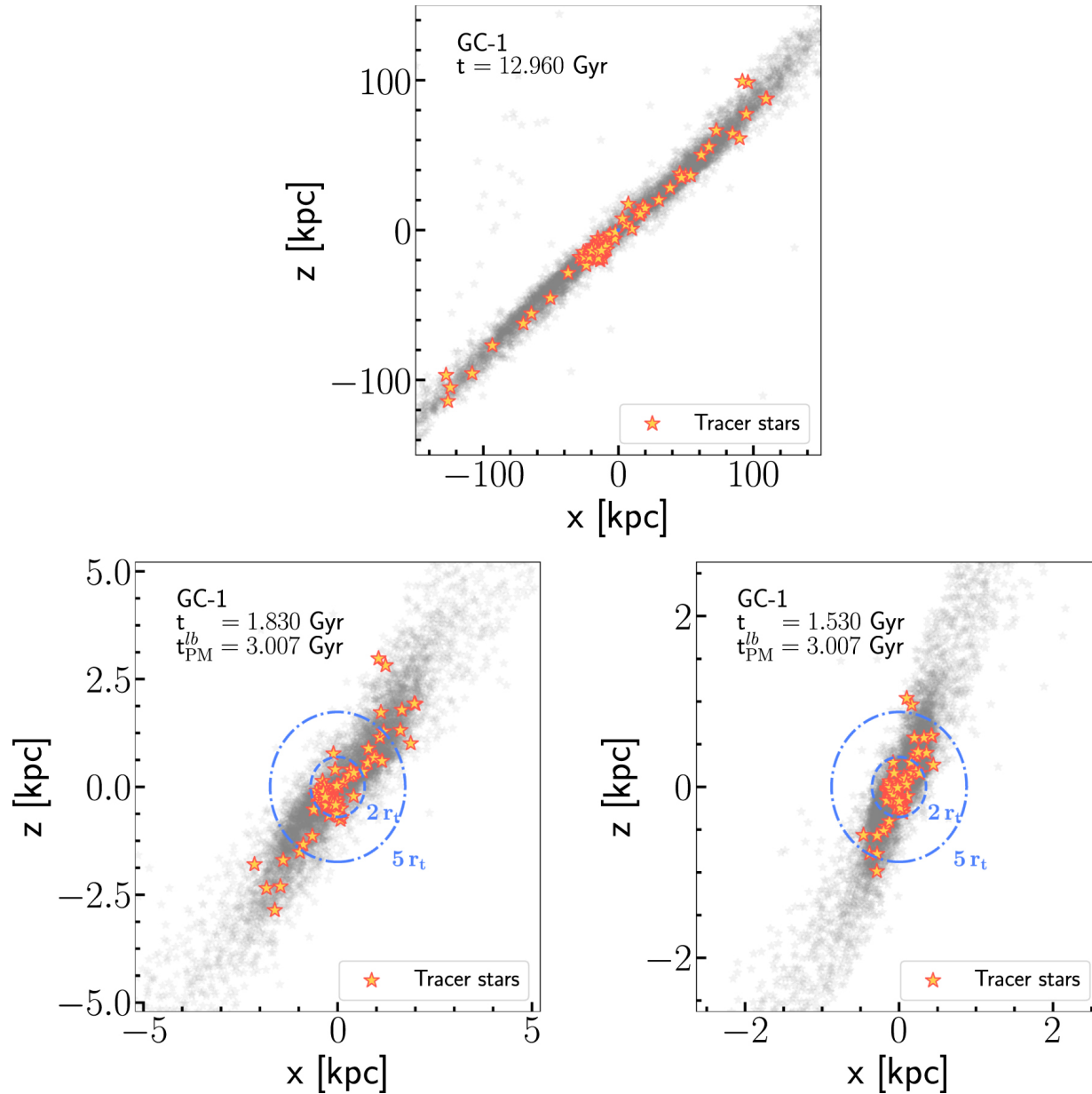
Figure 3. from Dating the Tidal Disruption of Globular Clusters with GAIA Data on Their Stellar Streams null 2018 APJL 859 L13 doi:10.3847/2041-8213/aac48c https://dx.doi.org/10.3847/2041-8213/aac48c © 2018. The American Astronomical Society. All rights reserved.
