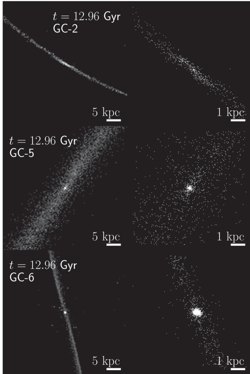
Figure 1. from Dating the Tidal Disruption of Globular Clusters with GAIA Data on Their Stellar Streams null 2018 APJL 859 L13 doi:10.3847/2041-8213/aac48c https://dx.doi.org/10.3847/2041-8213/aac48c © 2018. The American Astronomical Society. All rights reserved.
