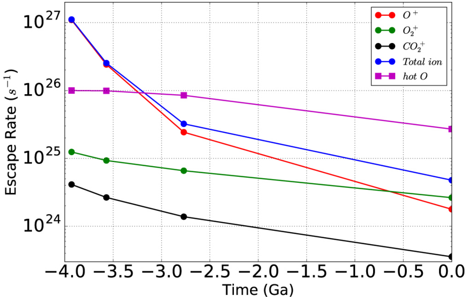
Figure 4. from Modeling Martian Atmospheric Losses over Time: Implications for Exoplanetary Climate Evolution and Habitability null 2018 APJL 859 L14 doi:10.3847/2041-8213/aac489 https://dx.doi.org/10.3847/2041-8213/aac489 © 2018. The American Astronomical Society. All rights reserved.
