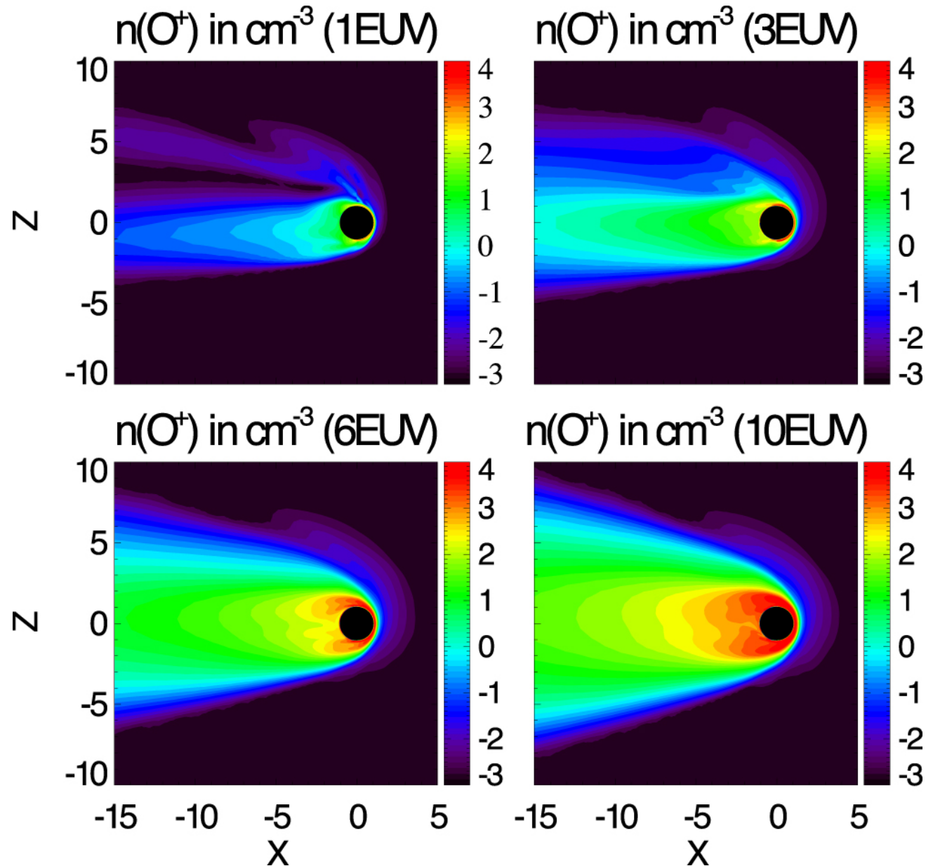
Figure 3. from Modeling Martian Atmospheric Losses over Time: Implications for Exoplanetary Climate Evolution and Habitability null 2018 APJL 859 L14 doi:10.3847/2041-8213/aac489 https://dx.doi.org/10.3847/2041-8213/aac489 © 2018. The American Astronomical Society. All rights reserved.
