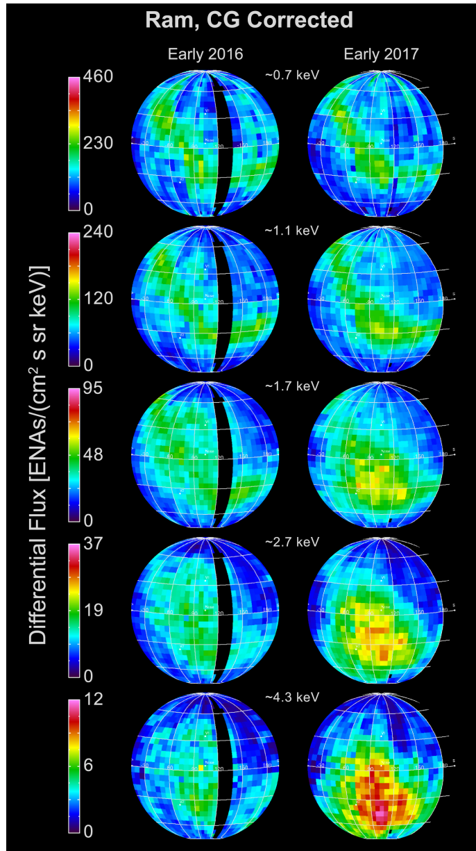
Figure 4. from Heliosphere Responds to a Large Solar Wind Intensification: Decisive Observations from IBEX null 2018 APJL 856 L10 doi:10.3847/2041-8213/aab611 https://dx.doi.org/10.3847/2041-8213/aab611 © 2018. The American Astronomical Society. All rights reserved.
