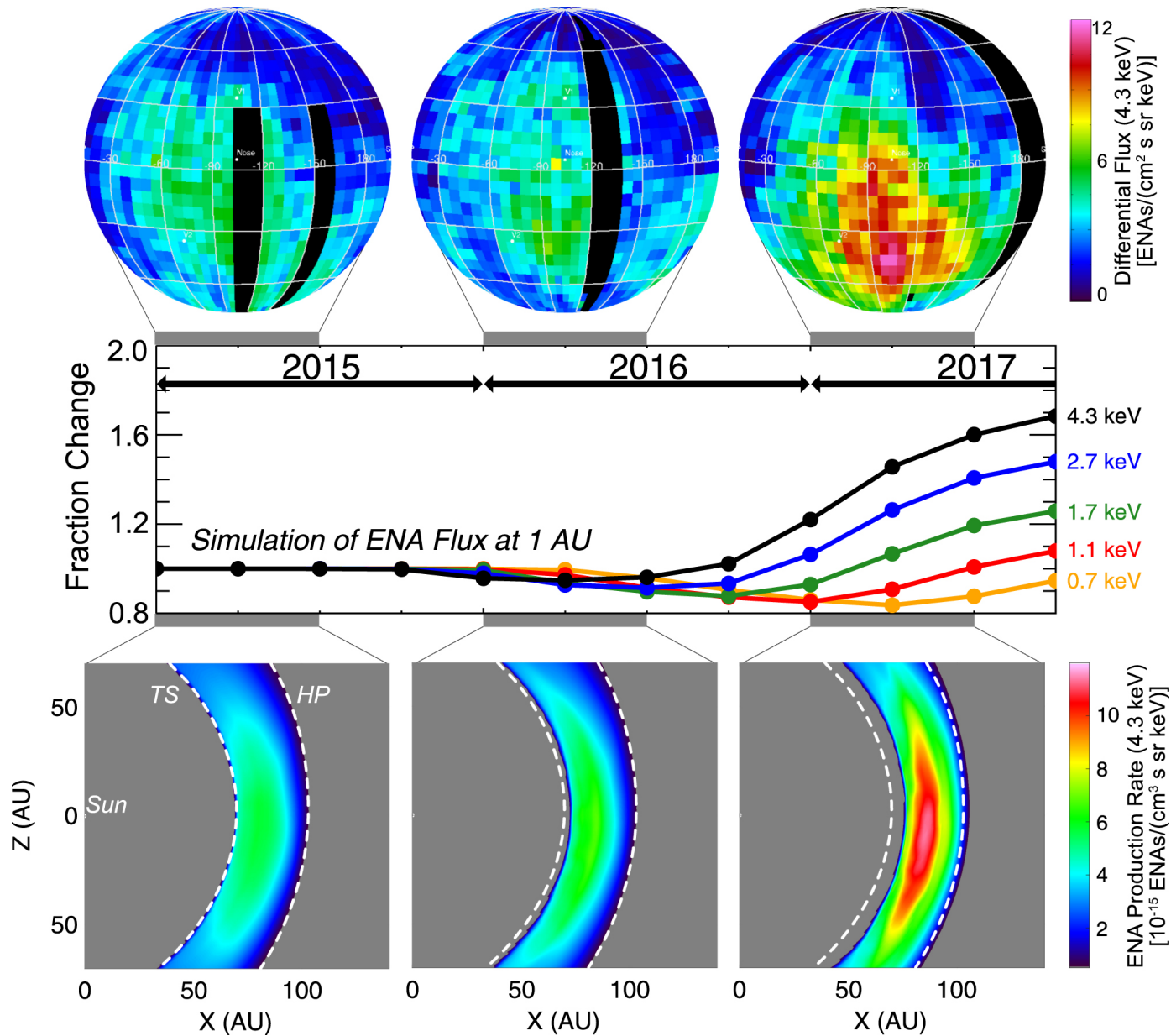
Figure 3. from Heliosphere Responds to a Large Solar Wind Intensification: Decisive Observations from IBEX null 2018 APJL 856 L10 doi:10.3847/2041-8213/aab611 https://dx.doi.org/10.3847/2041-8213/aab611 © 2018. The American Astronomical Society. All rights reserved.
