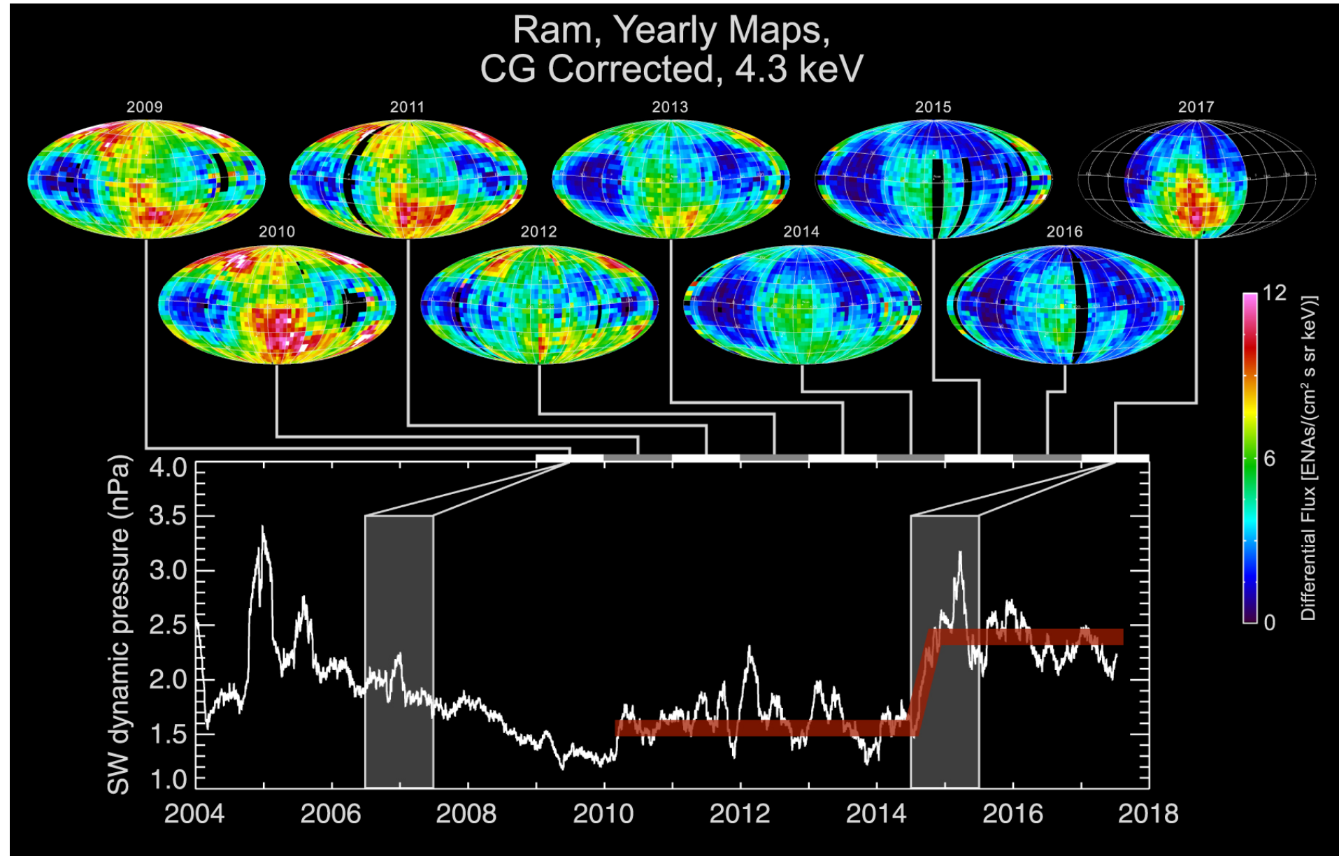
Figure 1. from Heliosphere Responds to a Large Solar Wind Intensification: Decisive Observations from IBEX null 2018 APJL 856 L10 doi:10.3847/2041-8213/aab611 https://dx.doi.org/10.3847/2041-8213/aab611 © 2018. The American Astronomical Society. All rights reserved.
