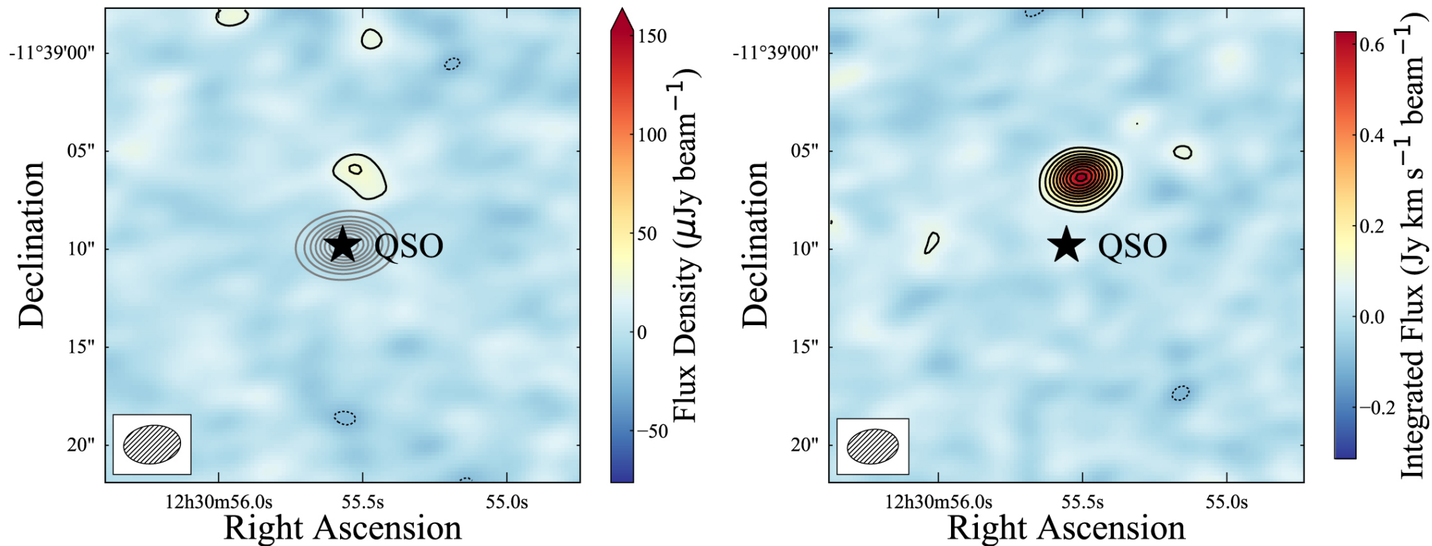
Figure 2. from Molecular Emission from a Galaxy Associated with a z = 2.2 Damped Ly Absorber null 2018 APJL 856 L12 doi:10.3847/2041-8213/aab5b1 https://dx.doi.org/10.3847/2041-8213/aab5b1 © 2018. The American Astronomical Society. All rights reserved.
