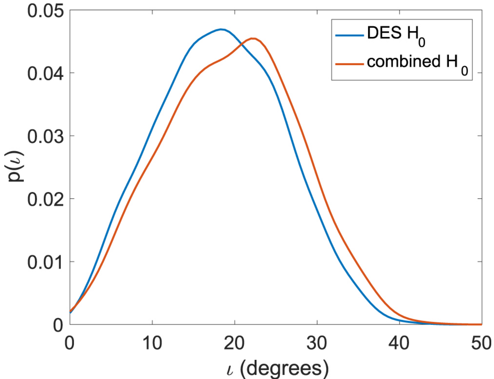
Figure 1. from The Orbit of GW170817 Was Inclined by Less Than 28^\circ to the Line of Sight null 2018 APJL 853 L12 doi:10.3847/2041-8213/aaa6c1 https://dx.doi.org/10.3847/2041-8213/aaa6c1 © 2018. The American Astronomical Society.
