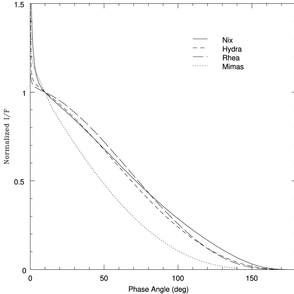
Figure 2. from Phase Curves of Nix and Hydra from the New Horizons Imaging Cameras null 2018 APJL 852 L35 doi:10.3847/2041-8213/aaa486 https://dx.doi.org/10.3847/2041-8213/aaa486 © 2018. The American Astronomical Society. All rights reserved.
