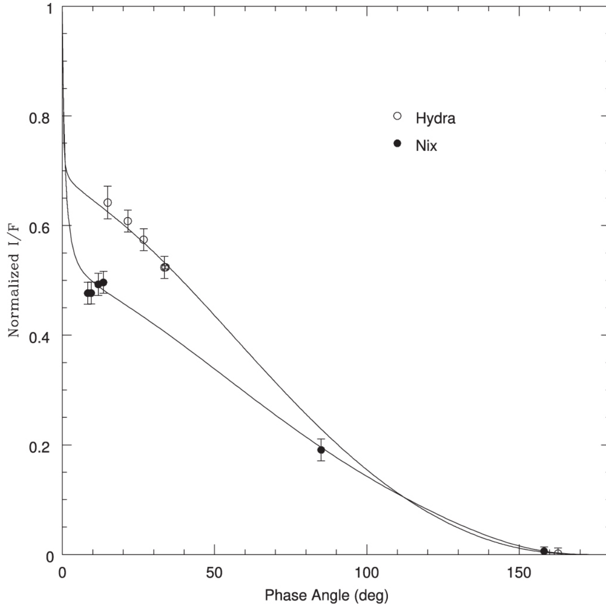
Figure 1. from Phase Curves of Nix and Hydra from the New Horizons Imaging Cameras null 2018 APJL 852 L35 doi:10.3847/2041-8213/aaa486 https://dx.doi.org/10.3847/2041-8213/aaa486 © 2018. The American Astronomical Society. All rights reserved.
