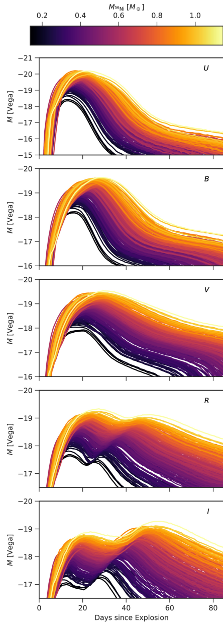
Figure 3. from Evidence for Sub-Chandrasekhar Mass Type Ia Supernovae from an Extensive Survey of Radiative Transfer Models null 2018 APJL 852 L33 doi:10.3847/2041-8213/aaa409 https://dx.doi.org/10.3847/2041-8213/aaa409 © 2018. The American Astronomical Society. All rights reserved.
