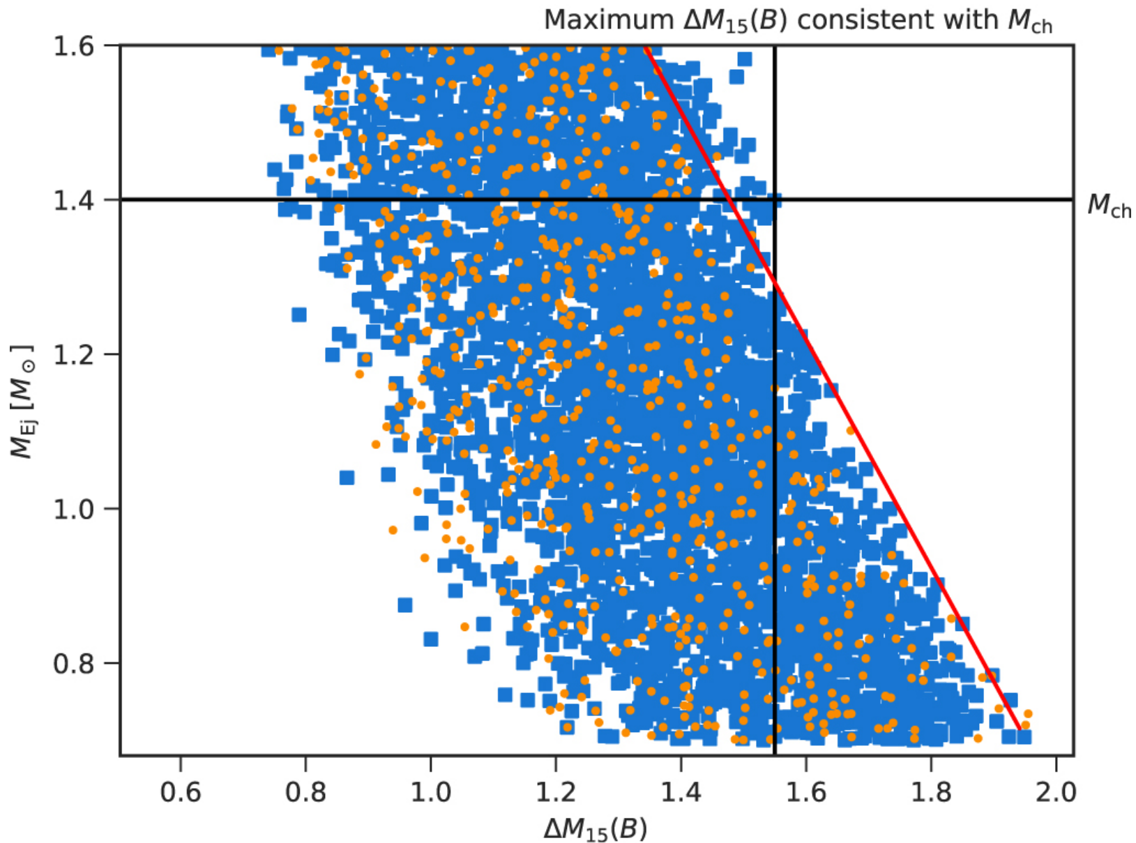
Figure 2. from Evidence for Sub-Chandrasekhar Mass Type Ia Supernovae from an Extensive Survey of Radiative Transfer Models null 2018 APJL 852 L33 doi:10.3847/2041-8213/aaa409 https://dx.doi.org/10.3847/2041-8213/aaa409 © 2018. The American Astronomical Society. All rights reserved.
