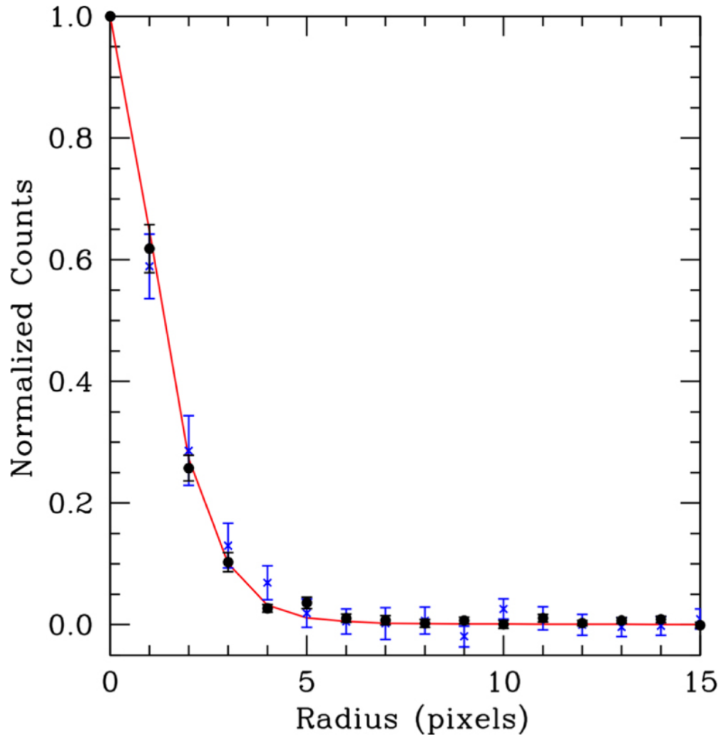
Figure 3. from On the Rotation Period and Shape of the Hyperbolic Asteroid 1I/'Oumuamua (2017 U1) from Its Lightcurve null 2017 APJL 851 L31 doi:10.3847/2041-8213/aa9d81 https://dx.doi.org/10.3847/2041-8213/aa9d81
