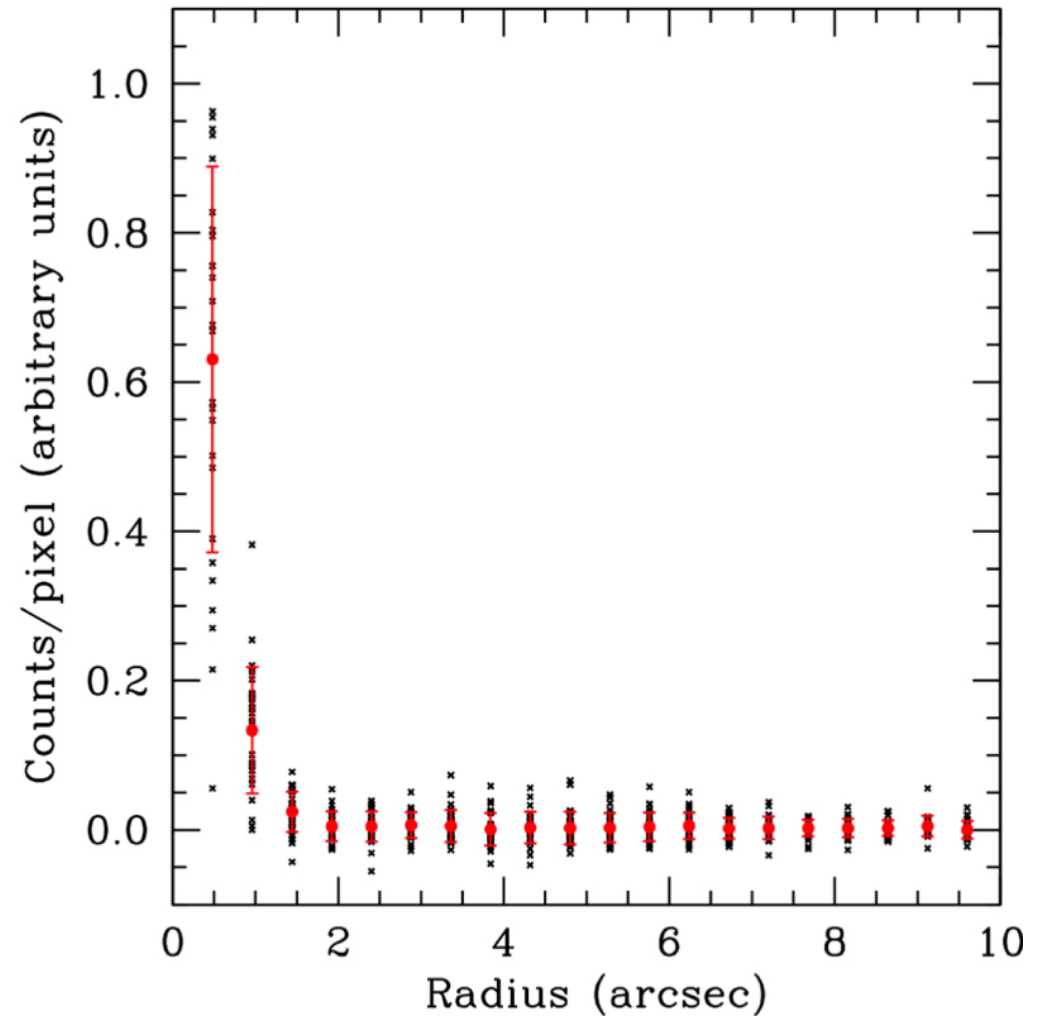
Figure 3. from On the Rotation Period and Shape of the Hyperbolic Asteroid 1I/'Oumuamua (2017 U1) from Its Lightcurve null 2017 APJL 851 L31 doi:10.3847/2041-8213/aa9d81 https://dx.doi.org/10.3847/2041-8213/aa9d81
