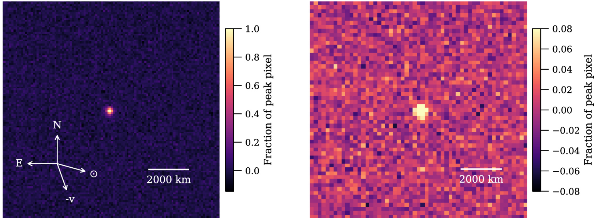
Figure 2. from On the Rotation Period and Shape of the Hyperbolic Asteroid 1I/'Oumuamua (2017 U1) from Its Lightcurve null 2017 APJL 851 L31 doi:10.3847/2041-8213/aa9d81 https://dx.doi.org/10.3847/2041-8213/aa9d81 © 2017. The American Astronomical Society. All rights reserved.
