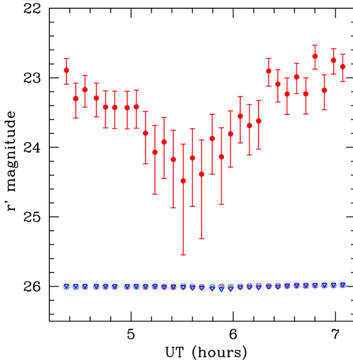
Figure 1. from On the Rotation Period and Shape of the Hyperbolic Asteroid 1I/'Oumuamua (2017 U1) from Its Lightcurve null 2017 APJL 851 L31 doi:10.3847/2041-8213/aa9d81 https://dx.doi.org/10.3847/2041-8213/aa9d81 © 2017. The American Astronomical Society. All rights reserved.
