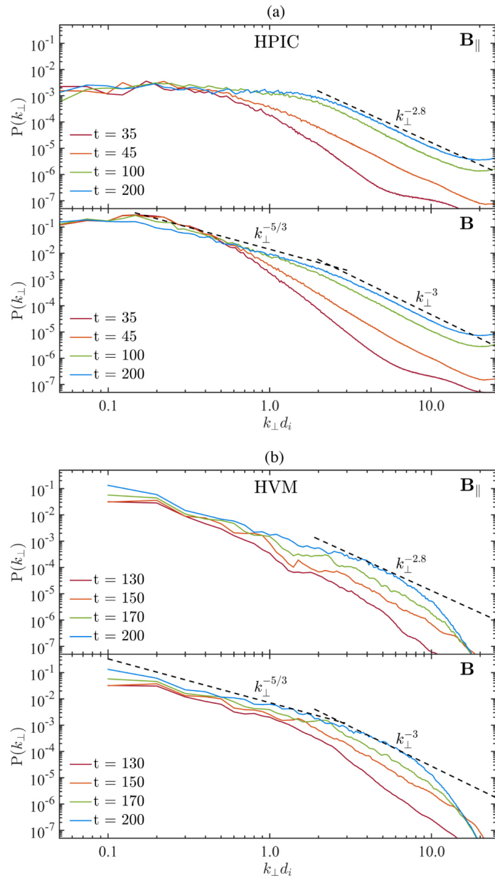
Figure 3. from Magnetic Reconnection as a Driver for a Sub-ion-scale Cascade in Plasma Turbulence null 2017 APJL 850 L16 doi:10.3847/2041-8213/aa93fb https://dx.doi.org/10.3847/2041-8213/aa93fb © 2017. The American Astronomical Society. All rights reserved.
