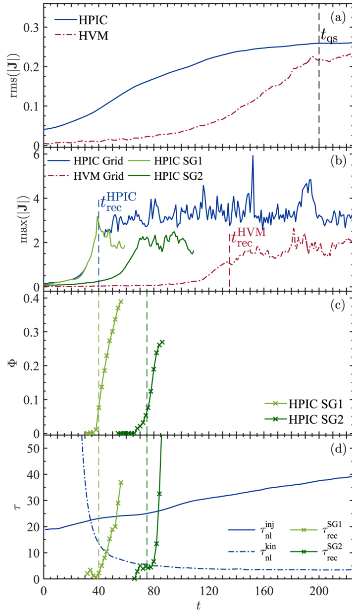
Figure 1. from Magnetic Reconnection as a Driver for a Sub-ion-scale Cascade in Plasma Turbulence null 2017 APJL 850 L16 doi:10.3847/2041-8213/aa93fb https://dx.doi.org/10.3847/2041-8213/aa93fb © 2017. The American Astronomical Society. All rights reserved.
