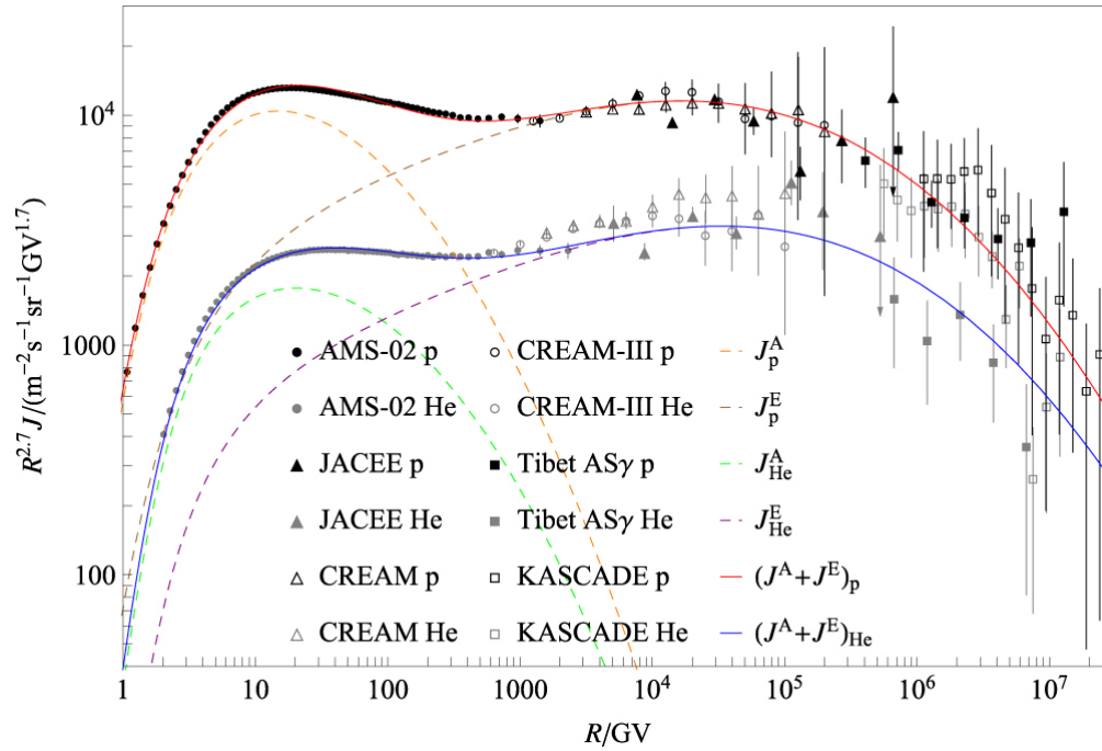
Figure 2. from Anomalous Distributions of Primary Cosmic Rays as Evidence for Time-dependent Particle Acceleration in Supernova Remnants null 2017 APJL 844 L3 doi:10.3847/2041-8213/aa7de1 https://dx.doi.org/10.3847/2041-8213/aa7de1 © 2017. The American Astronomical Society. All rights reserved.
