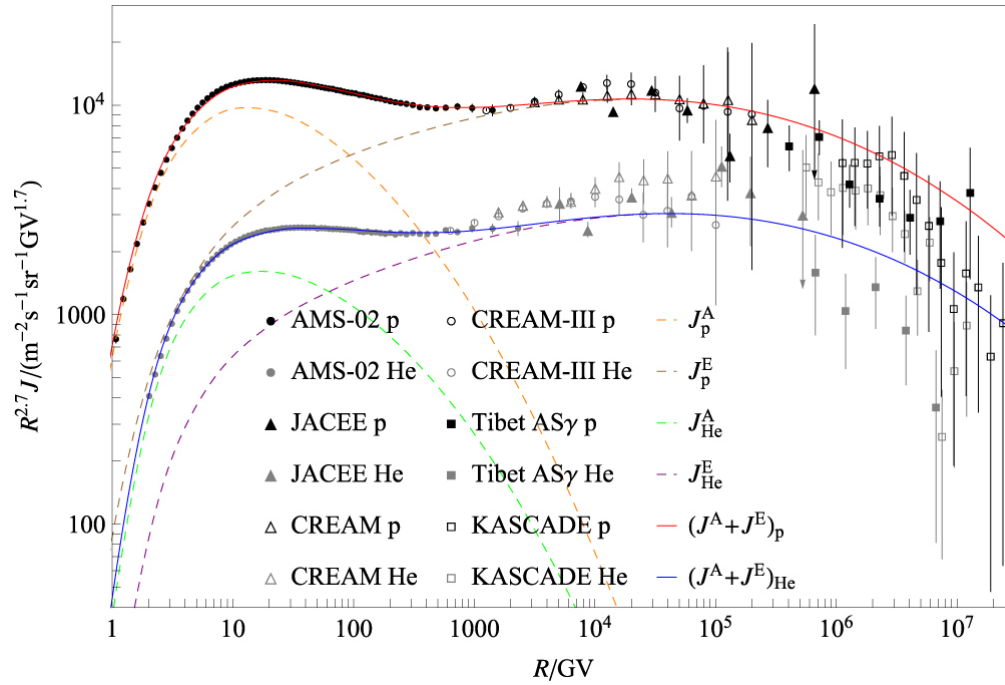
Figure 1. from Anomalous Distributions of Primary Cosmic Rays as Evidence for Time-dependent Particle Acceleration in Supernova Remnants null 2017 APJL 844 L3 doi:10.3847/2041-8213/aa7de1 https://dx.doi.org/10.3847/2041-8213/aa7de1 © 2017. The American Astronomical Society. All rights reserved.
