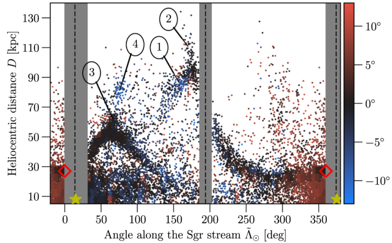
Figure 1. from The >100 kpc Distant Spur of the Sagittarius Stream and the Outer Virgo Overdensity, as Seen in PS1 RR Lyrae Stars null 2017 APJL 844 L4 doi:10.3847/2041-8213/aa7c61 https://dx.doi.org/10.3847/2041-8213/aa7c61 © 2017. The American Astronomical Society. All rights reserved.
