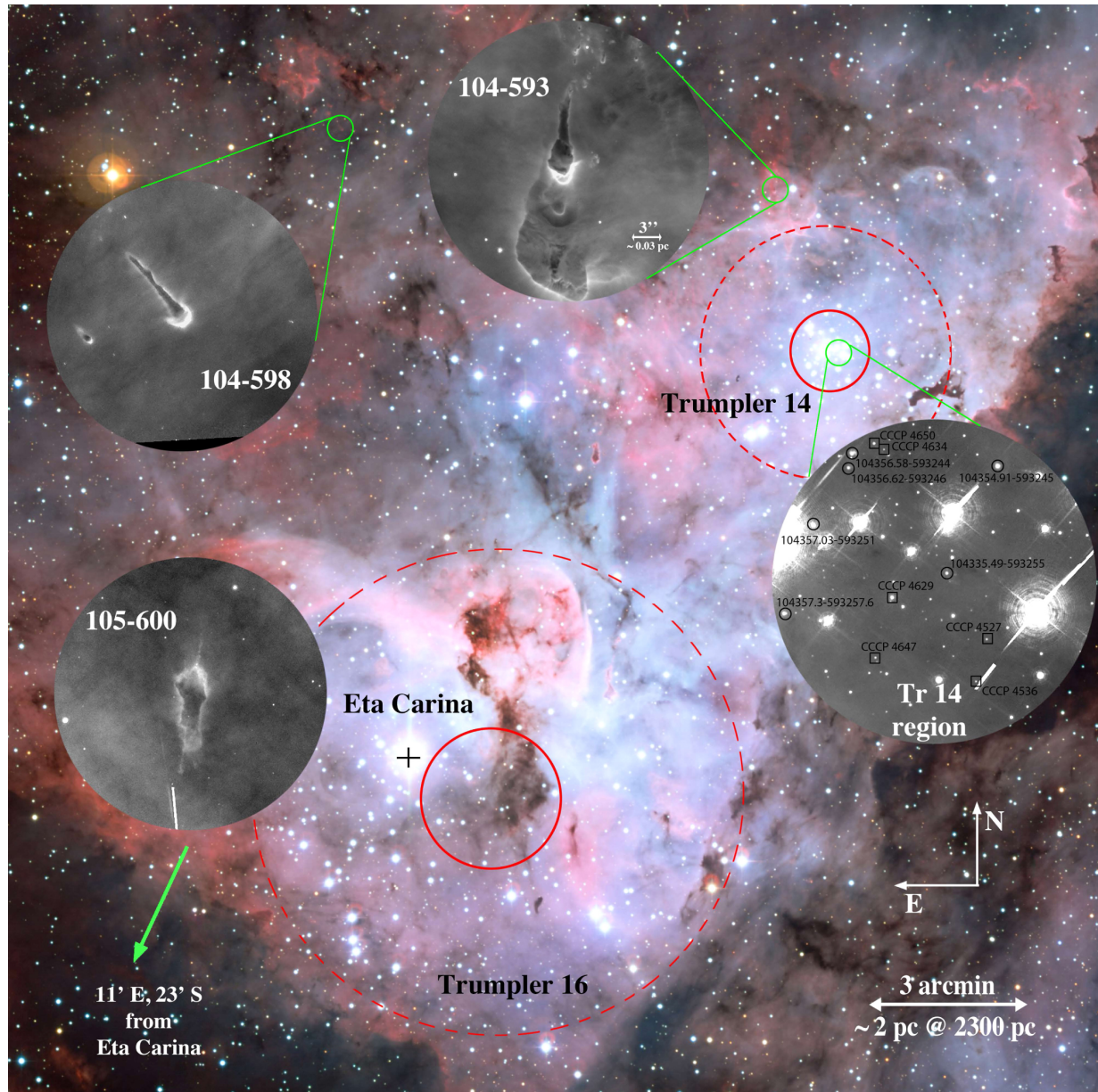
Figure 1. from PROTOPLANETARY DISKS IN THE HOSTILE ENVIRONMENT OF CARINA null 2016 APJL 825 L16 doi:10.3847/2041-8205/825/1/L16 https://dx.doi.org/10.3847/2041-8205/825/1/L16 © 2016. The American Astronomical Society. All rights reserved.
