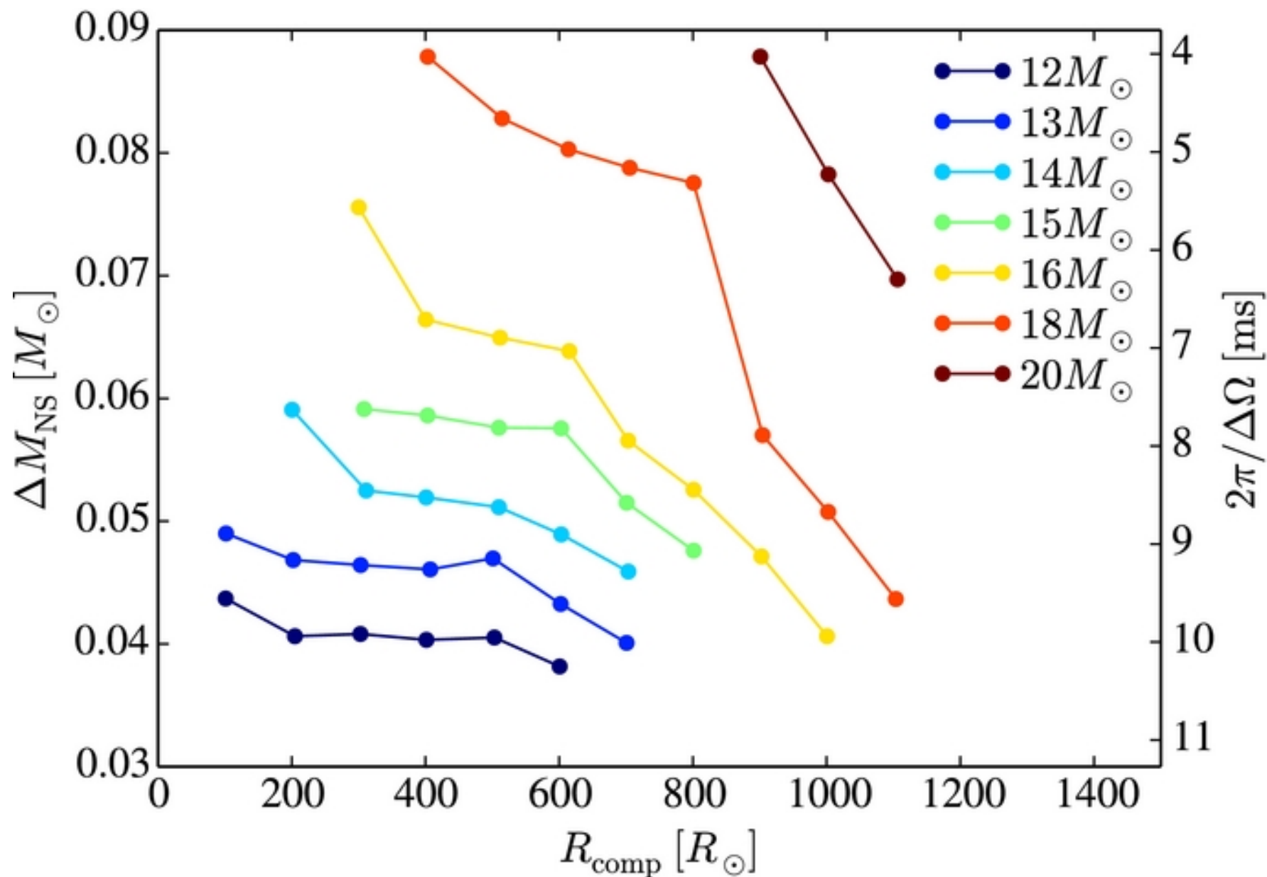
Figure 4. from On the Accretion-fed Growth of Neutron Stars during Common Envelope MacLeod & Ramirez-Ruiz 2015 ApJL 798 L19 doi:10.1088/2041-8205/798/1/L19 https://dx.doi.org/10.1088/2041-8205/798/1/L19 © 2015. The American Astronomical Society. All rights reserved.
