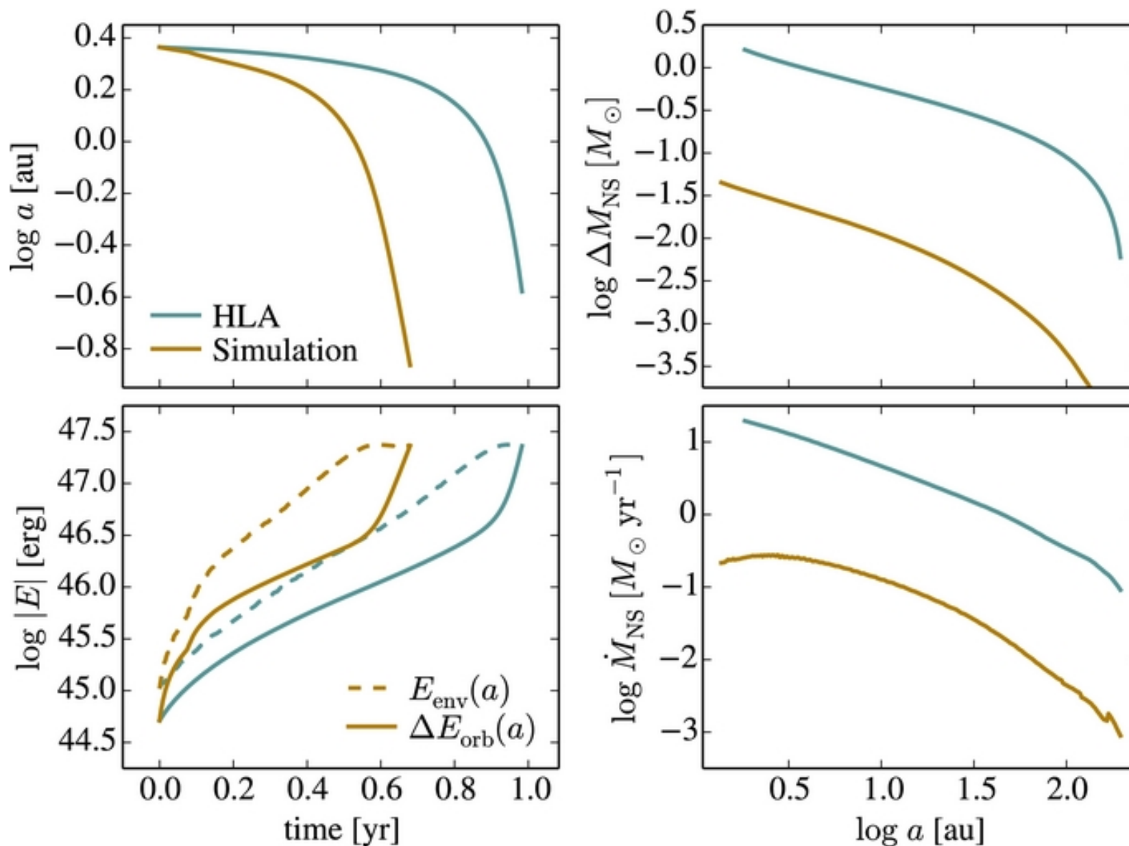
Figure 3. from On the Accretion-fed Growth of Neutron Stars during Common Envelope MacLeod & Ramirez-Ruiz 2015 ApJL 798 L19 doi:10.1088/2041-8205/798/1/L19 https://dx.doi.org/10.1088/2041-8205/798/1/L19 © 2015. The American Astronomical Society. All rights reserved.
