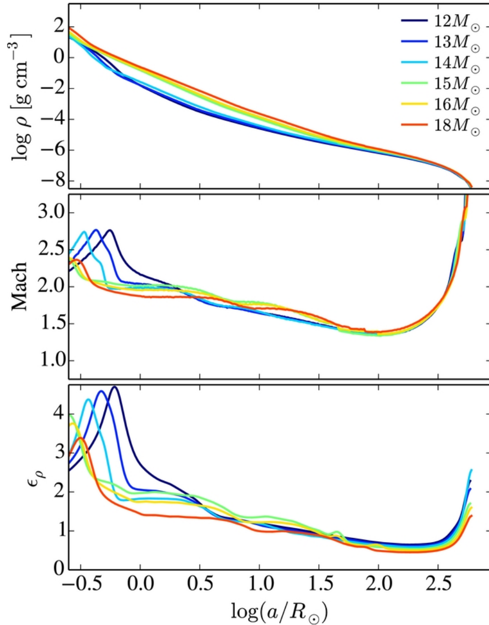
Figure 2. from On the Accretion-fed Growth of Neutron Stars during Common Envelope MacLeod & Ramirez-Ruiz 2015 ApJL 798 L19 doi:10.1088/2041-8205/798/1/L19 https://dx.doi.org/10.1088/2041-8205/798/1/L19 © 2015. The American Astronomical Society. All rights reserved.
