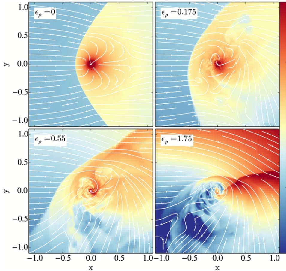
Figure 1. from On the Accretion-fed Growth of Neutron Stars during Common Envelope MacLeod & Ramirez-Ruiz 2015 ApJL 798 L19 doi:10.1088/2041-8205/798/1/L19 https://dx.doi.org/10.1088/2041-8205/798/1/L19 © 2015. The American Astronomical Society. All rights reserved.
