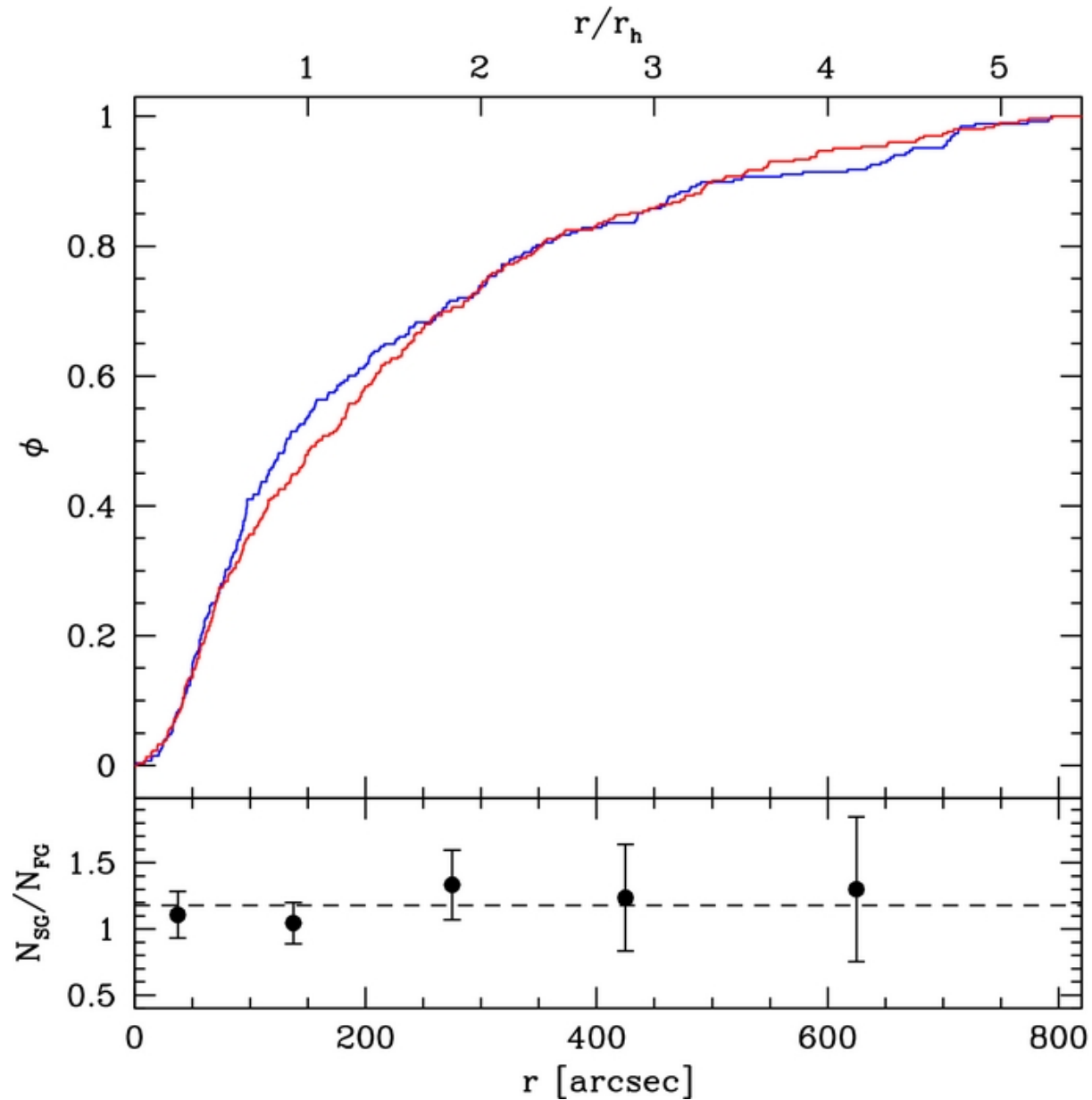
Figure 5. from First Evidence of Fully Spatially Mixed First and Second Generations in Globular Clusters: The Case of NGC 6362 Dalessandro et al. 2014 ApJL 791 L4 doi:10.1088/2041-8205/791/1/L4 https://dx.doi.org/10.1088/2041-8205/791/1/L4 © 2014. The American Astronomical Society. All rights reserved.
