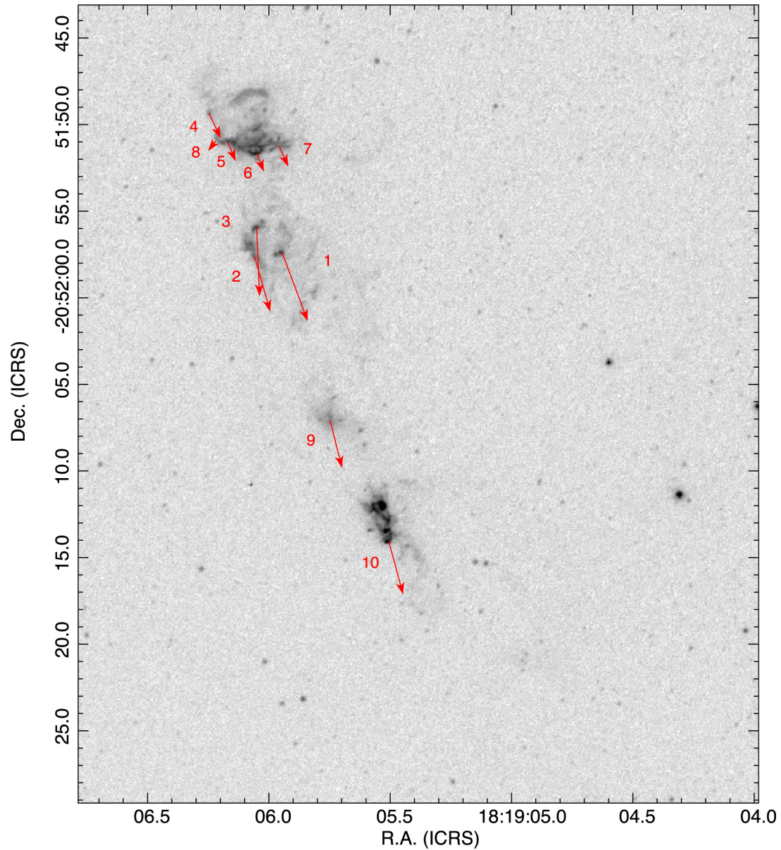
Figure 7. from John Bally and Bo Reipurth 2023 Astrophys. J. 958 doi:10.3847/1538-4357/acf028 https://dx.doi.org/10.3847/1538-4357/acf028 © 2023. The Author(s). Published by the American Astronomical Society.
