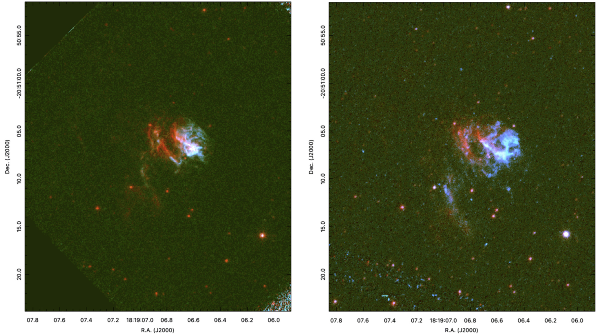
Figure 26. from John Bally and Bo Reipurth 2023 Astrophys. J. 958 doi:10.3847/1538-4357/acf028 https://dx.doi.org/10.3847/1538-4357/acf028 © 2023. The Author(s). Published by the American Astronomical Society.
