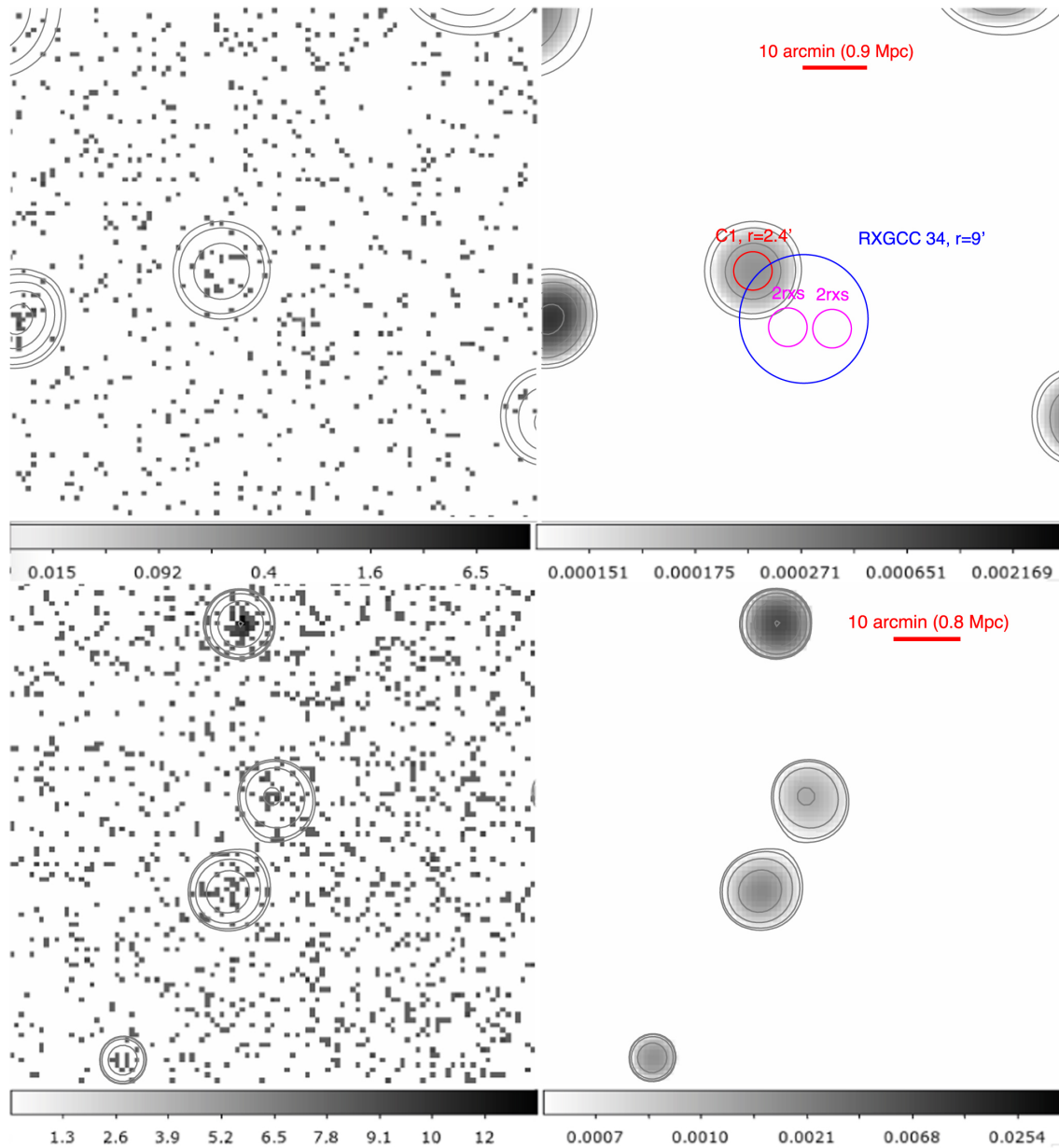
Figure 1. from Kaiyuan Chen et al 2022 Astrophys. J. 940 doi:10.3847/1538-4357/ac9b44 http://dx.doi.org/10.3847/1538-4357/ac9b44 © 2022. The Author(s). Published by the American Astronomical Society.
